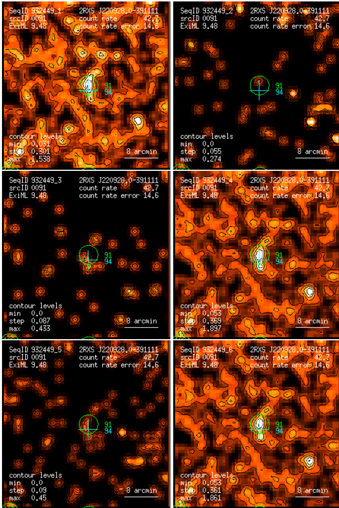
Figure 91: RASS 932449: detection 0091: band rate images, Gaussian filter: (1) PSPC channels 11 – 41, (2) 52 – 90, (3) 91 – 201, (4) 11 – 235, (5) 52 – 201, (6) 11 – 201. Broad band rates in counts/ks. Band rate contour levels in counts/ks/arcmin 2 .
