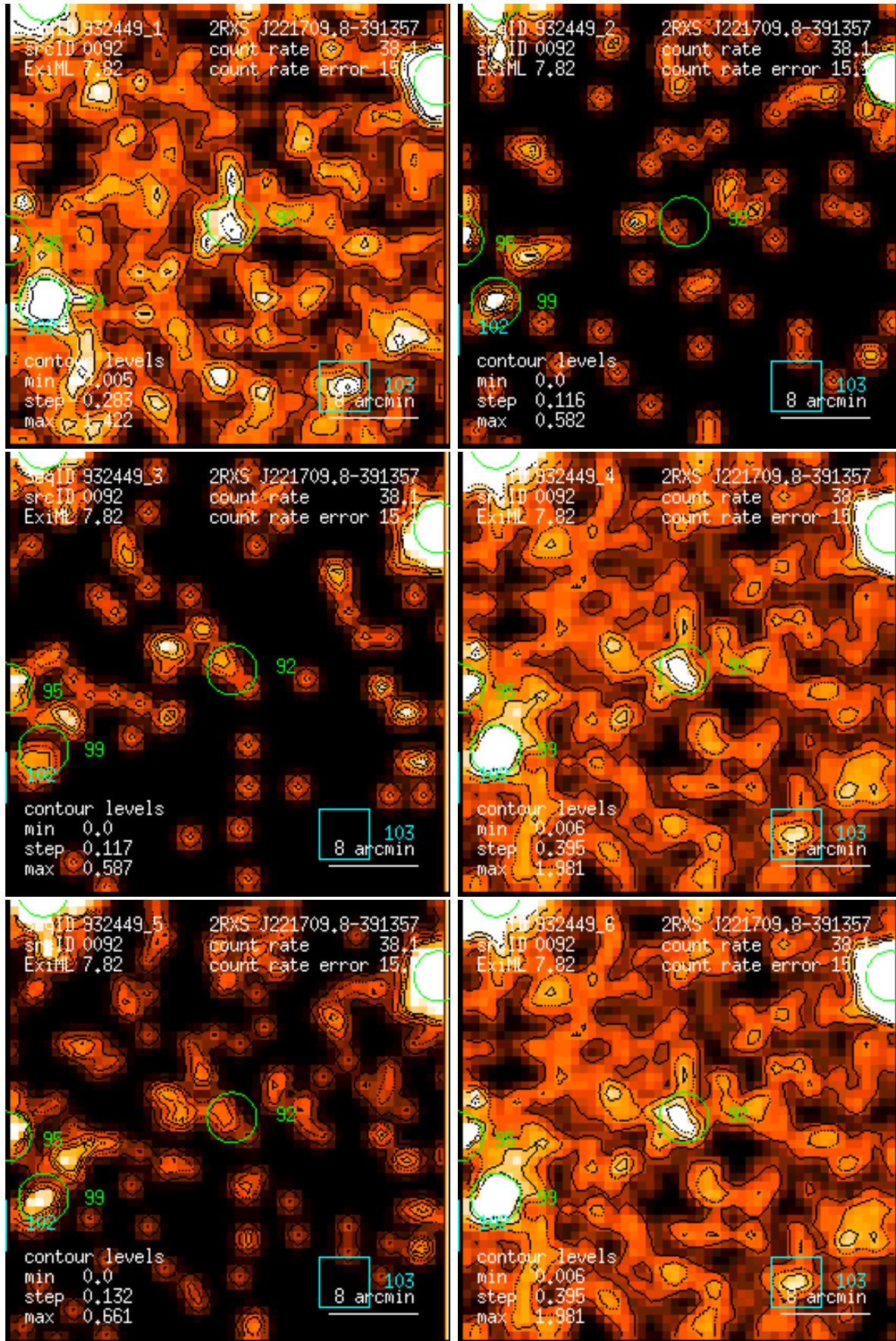
Figure 92: RASS 932449: detection 0092: band rate images, Gaussian filter: (1) PSPC channels 11 – 41, (2) 52 – 90, (3) 91 – 201, (4) 11 – 235, (5) 52 – 201, (6) 11 – 201. Broad band rates in counts/ks. Band rate contour levels in counts/ks/arcmin 2 .
