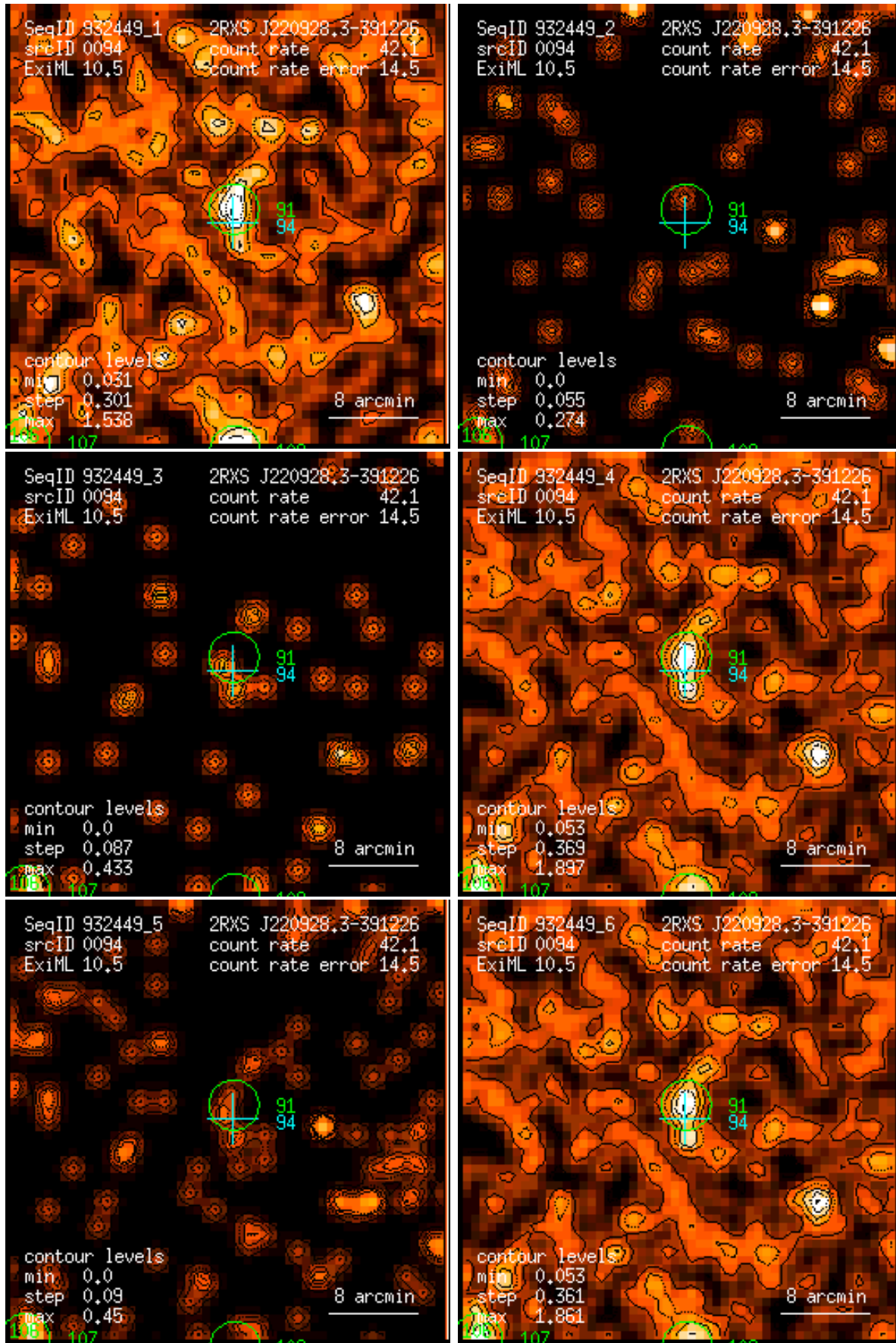
Figure 94: RASS 932449: detection 0094: band rate images, Gaussian filter: (1) PSPC channels 11 – 41, (2) 52 – 90, (3) 91 – 201, (4) 11 – 235, (5) 52 – 201, (6) 11 – 201. Broad band rates in counts/ks. Band rate contour levels in counts/ks/arcmin 2 .
