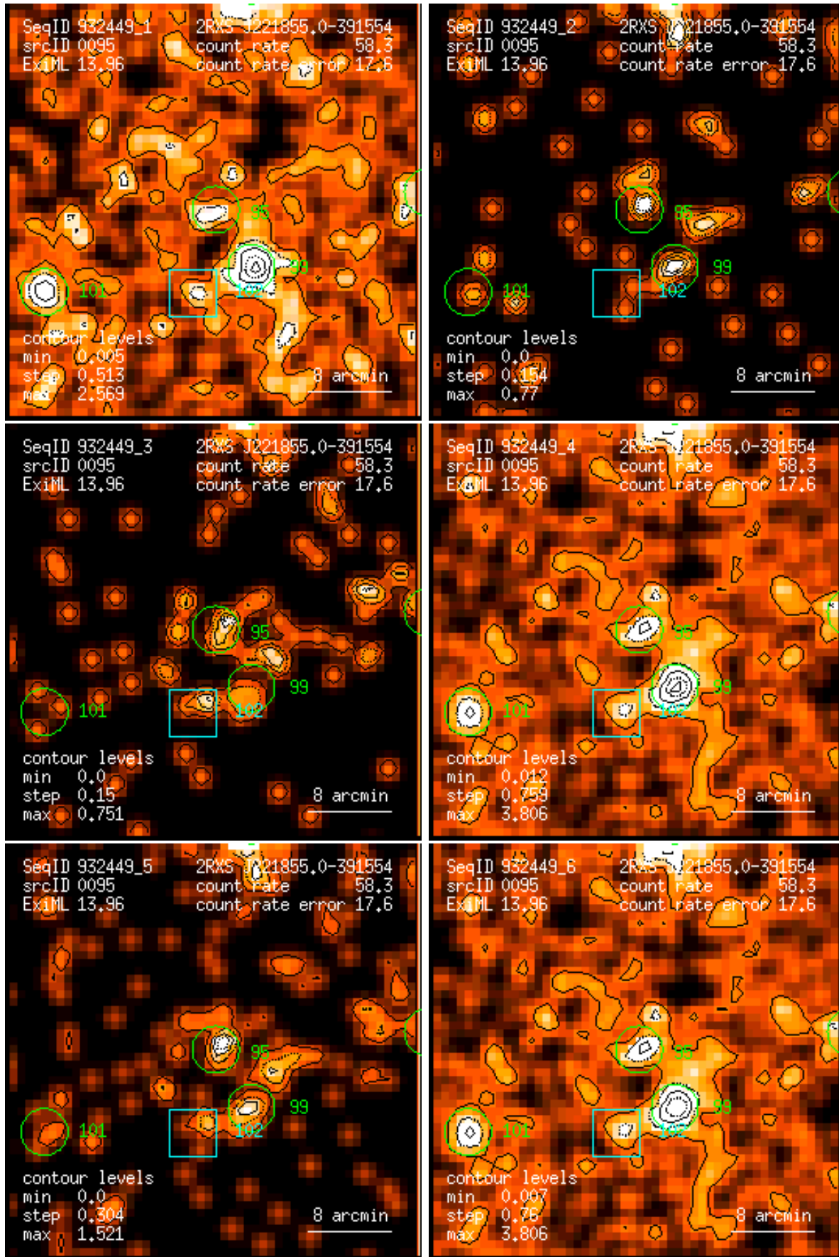
Figure 95: RASS 932449: detection 0095: band rate images, Gaussian filter: (1) PSPC channels 11 – 41, (2) 52 – 90, (3) 91 – 201, (4) 11 – 235, (5) 52 – 201, (6) 11 – 201. Broad band rates in counts/ks. Band rate contour levels in counts/ks/arcmin 2 .
