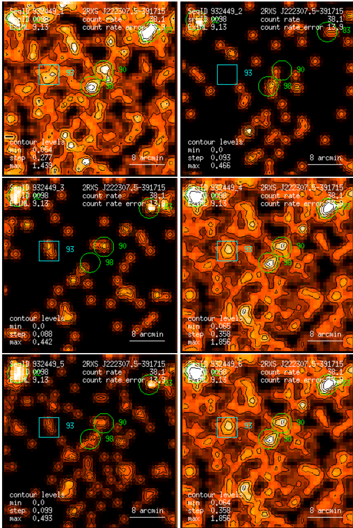
Figure 98: RASS 932449: detection 0098: band rate images, Gaussian filter: (1) PSPC channels 11 – 41, (2) 52 – 90, (3) 91 – 201, (4) 11 – 235, (5) 52 – 201, (6) 11 – 201. Broad band rates in counts/ks. Band rate contour levels in counts/ks/arcmin 2 .
