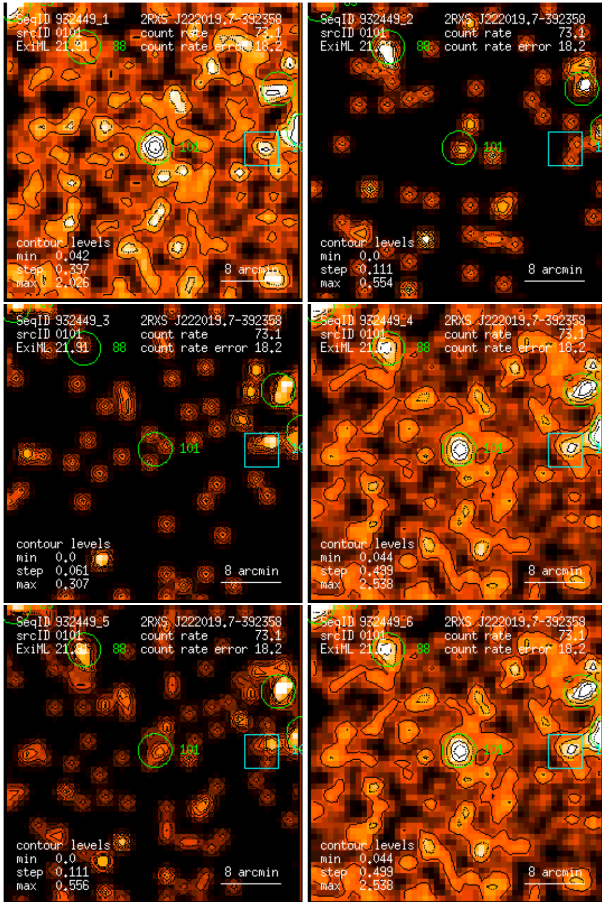
Figure 101: RASS 932449: detection 0101: band rate images, Gaussian filter: (1) PSPC channels 11 – 41, (2) 52 – 90, (3) 91 – 201, (4) 11 – 235, (5) 52 – 201, (6) 11 – 201. Broad band rates in counts/ks. Band rate contour levels in counts/ks/arcmin 2 .
