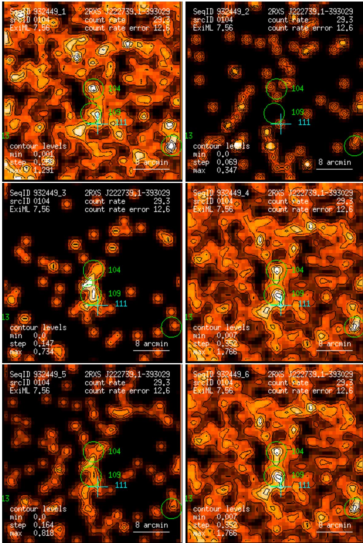
Figure 104: RASS 932449: detection 0104: band rate images, Gaussian filter: (1) PSPC channels 11 – 41, (2) 52 – 90, (3) 91 – 201, (4) 11 – 235, (5) 52 – 201, (6) 11 – 201. Broad band rates in counts/ks. Band rate contour levels in counts/ks/arcmin 2 .
