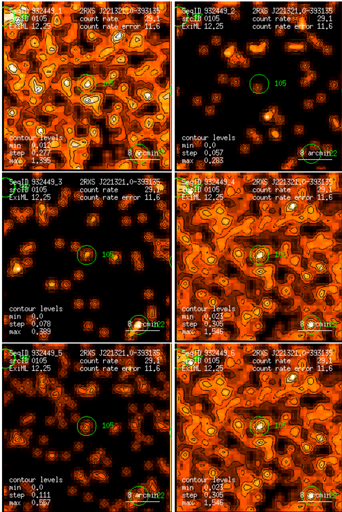
Figure 105: RASS 932449: detection 0105: band rate images, Gaussian filter: (1) PSPC channels 11 – 41, (2) 52 – 90, (3) 91 – 201, (4) 11 – 235, (5) 52 – 201, (6) 11 – 201. Broad band rates in counts/ks. Band rate contour levels in counts/ks/arcmin 2 .
