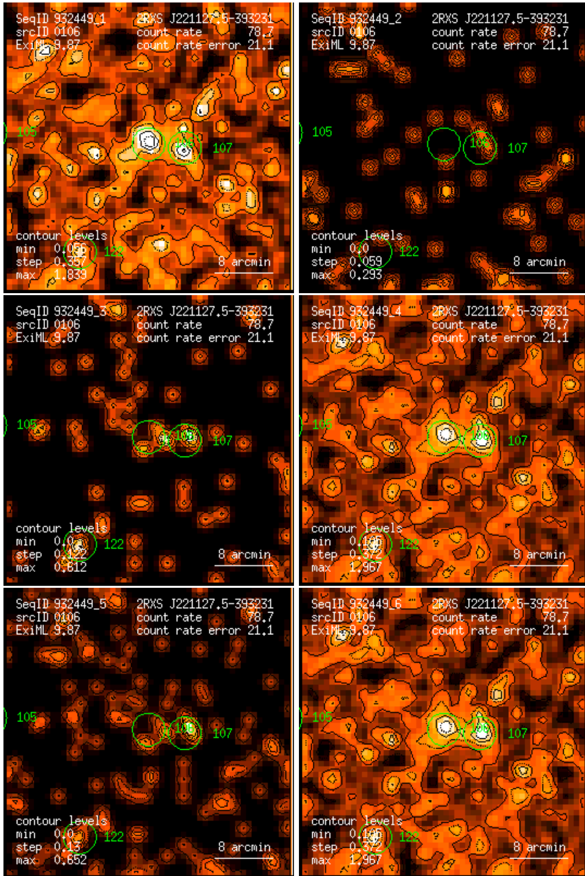
Figure 106: RASS 932449: detection 0106: band rate images, Gaussian filter: (1) PSPC channels 11 – 41, (2) 52 – 90, (3) 91 – 201, (4) 11 – 235, (5) 52 – 201, (6) 11 – 201. Broad band rates in counts/ks. Band rate contour levels in counts/ks/arcmin 2 .
