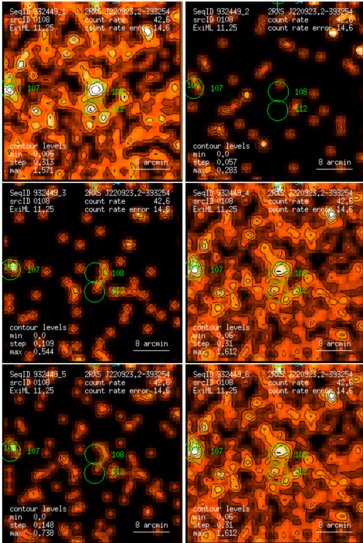
Figure 108: RASS 932449: detection 0108: band rate images, Gaussian filter: (1) PSPC channels 11 – 41, (2) 52 – 90, (3) 91 – 201, (4) 11 – 235, (5) 52 – 201, (6) 11 – 201. Broad band rates in counts/ks. Band rate contour levels in counts/ks/arcmin 2 .
