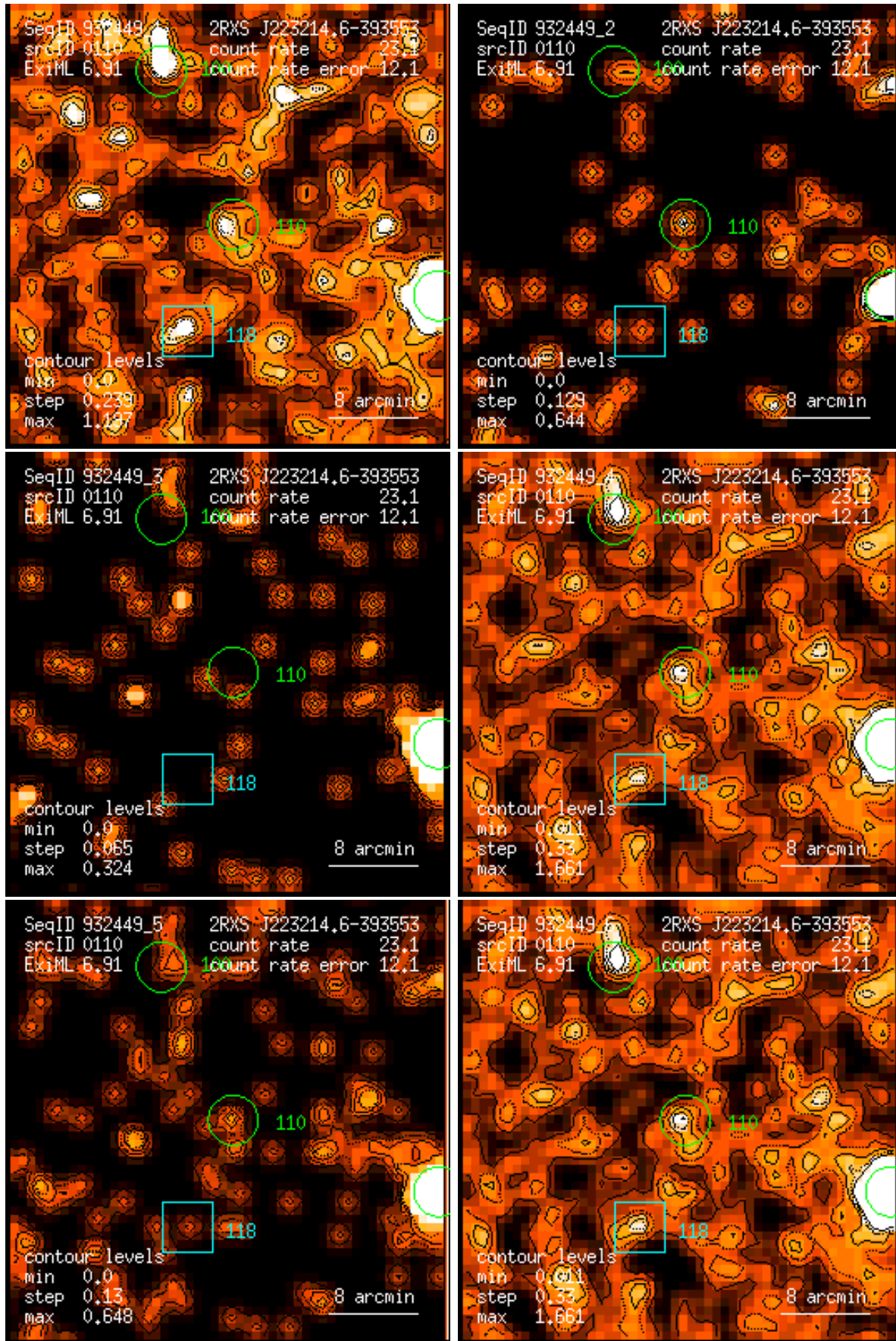
Figure 110: RASS 932449: detection 0110: band rate images, Gaussian filter: (1) PSPC channels 11 – 41, (2) 52 – 90, (3) 91 – 201, (4) 11 – 235, (5) 52 – 201, (6) 11 – 201. Broad band rates in counts/ks. Band rate contour levels in counts/ks/arcmin 2 .
