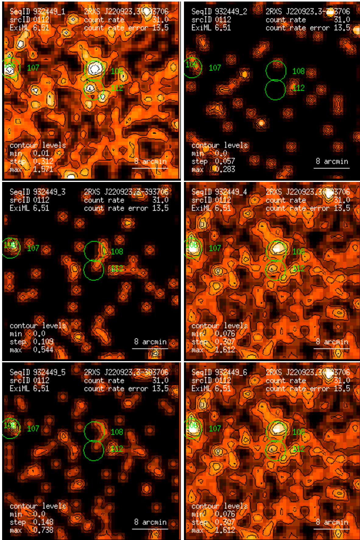
Figure 112: RASS 932449: detection 0112: band rate images, Gaussian filter: (1) PSPC channels 11 – 41, (2) 52 – 90, (3) 91 – 201, (4) 11 – 235, (5) 52 – 201, (6) 11 – 201. Broad band rates in counts/ks. Band rate contour levels in counts/ks/arcmin 2 .
