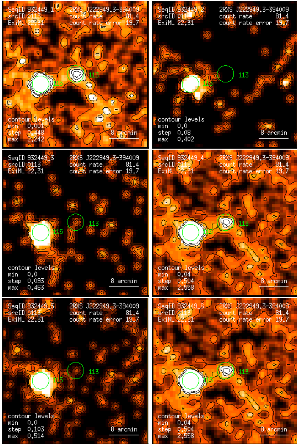
Figure 113: RASS 932449: detection 0113: band rate images, Gaussian filter: (1) PSPC channels 11 – 41, (2) 52 – 90, (3) 91 – 201, (4) 11 – 235, (5) 52 – 201, (6) 11 – 201. Broad band rates in counts/ks. Band rate contour levels in counts/ks/arcmin 2 .
