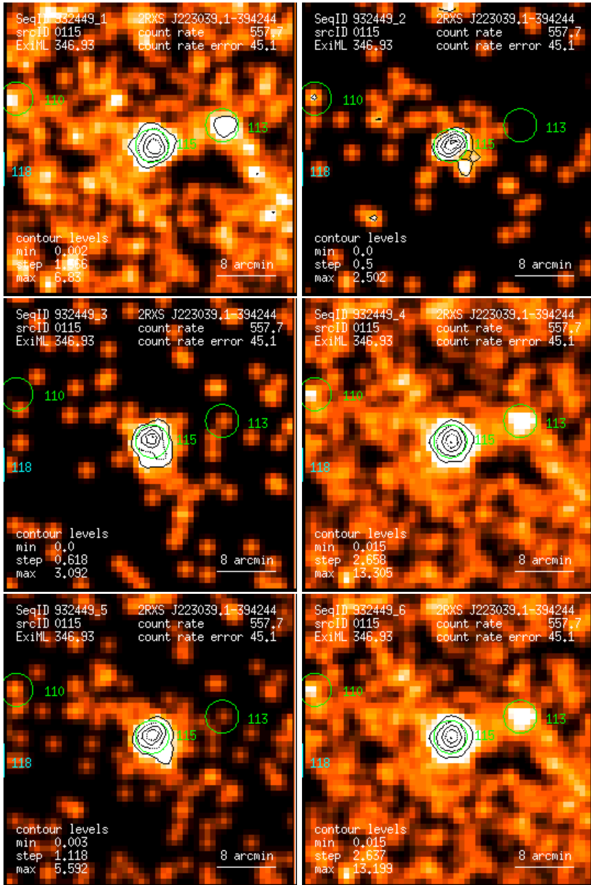
Figure 115: RASS 932449: detection 0115: band rate images, Gaussian filter: (1) PSPC channels 11 – 41, (2) 52 – 90, (3) 91 – 201, (4) 11 – 235, (5) 52 – 201, (6) 11 – 201. Broad band rates in counts/ks. Band rate contour levels in counts/ks/arcmin 2 .
