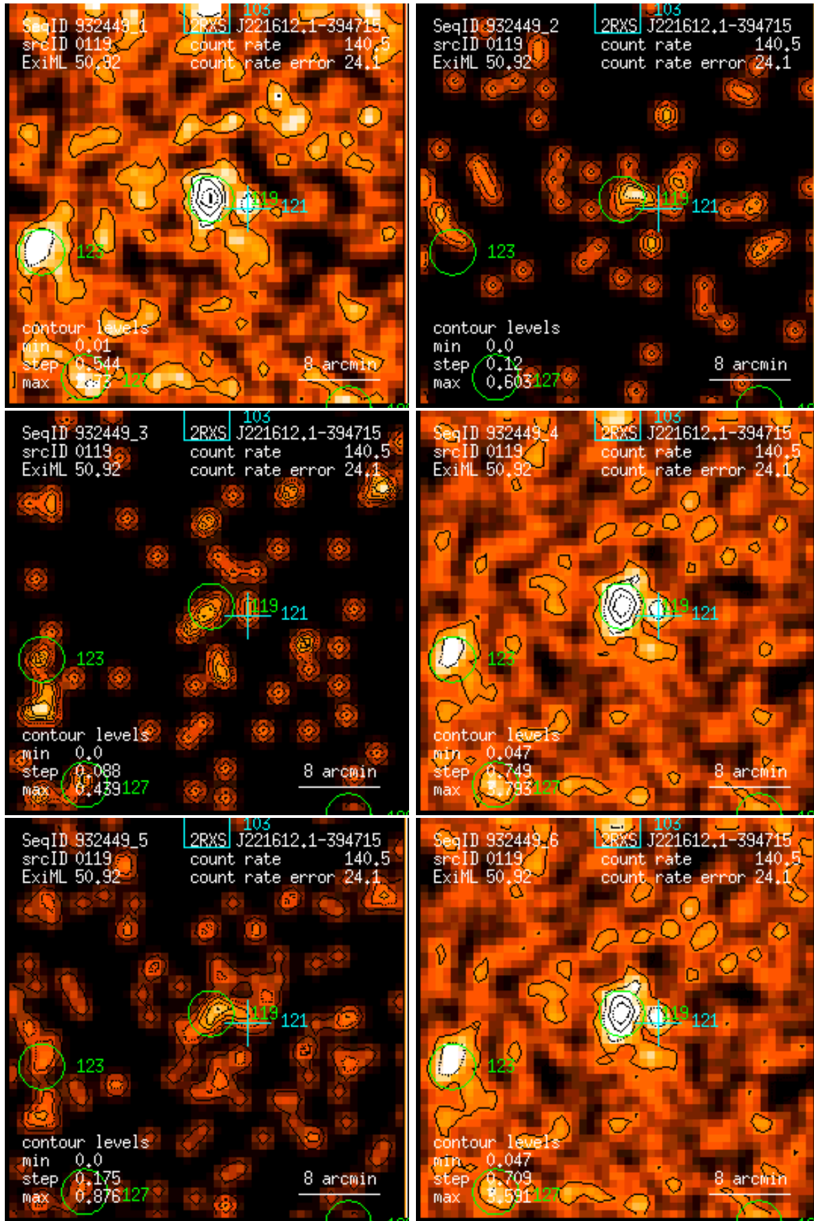
Figure 119: RASS 932449: detection 0119: band rate images, Gaussian filter: (1) PSPC channels 11 – 41, (2) 52 – 90, (3) 91 – 201, (4) 11 – 235, (5) 52 – 201, (6) 11 – 201. Broad band rates in counts/ks. Band rate contour levels in counts/ks/arcmin 2 .
