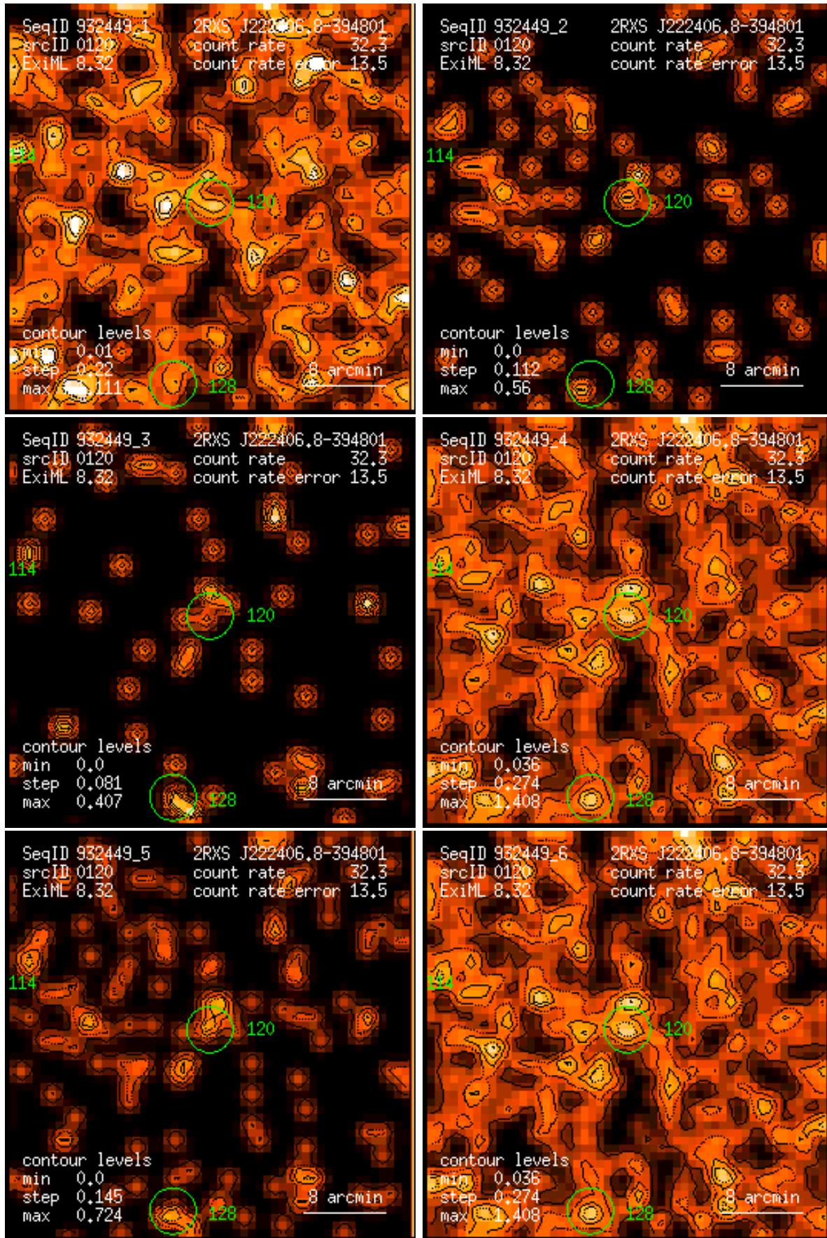
Figure 120: RASS 932449: detection 0120: band rate images, Gaussian filter: (1) PSPC channels 11 – 41, (2) 52 – 90, (3) 91 – 201, (4) 11 – 235, (5) 52 – 201, (6) 11 – 201. Broad band rates in counts/ks. Band rate contour levels in counts/ks/arcmin 2 .
