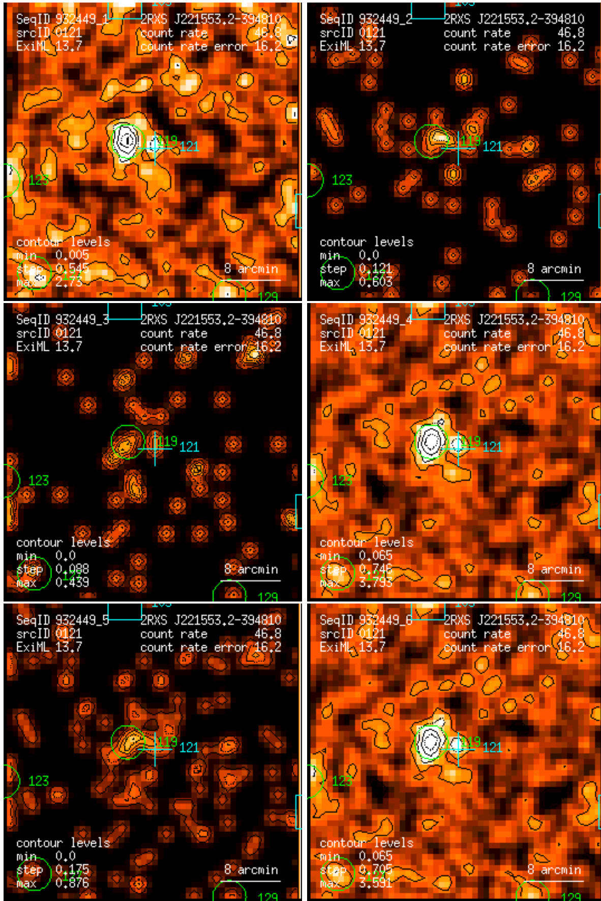
Figure 121: RASS 932449: detection 0121: band rate images, Gaussian filter: (1) PSPC channels 11 – 41, (2) 52 – 90, (3) 91 – 201, (4) 11 – 235, (5) 52 – 201, (6) 11 – 201. Broad band rates in counts/ks. Band rate contour levels in counts/ks/arcmin 2 .
