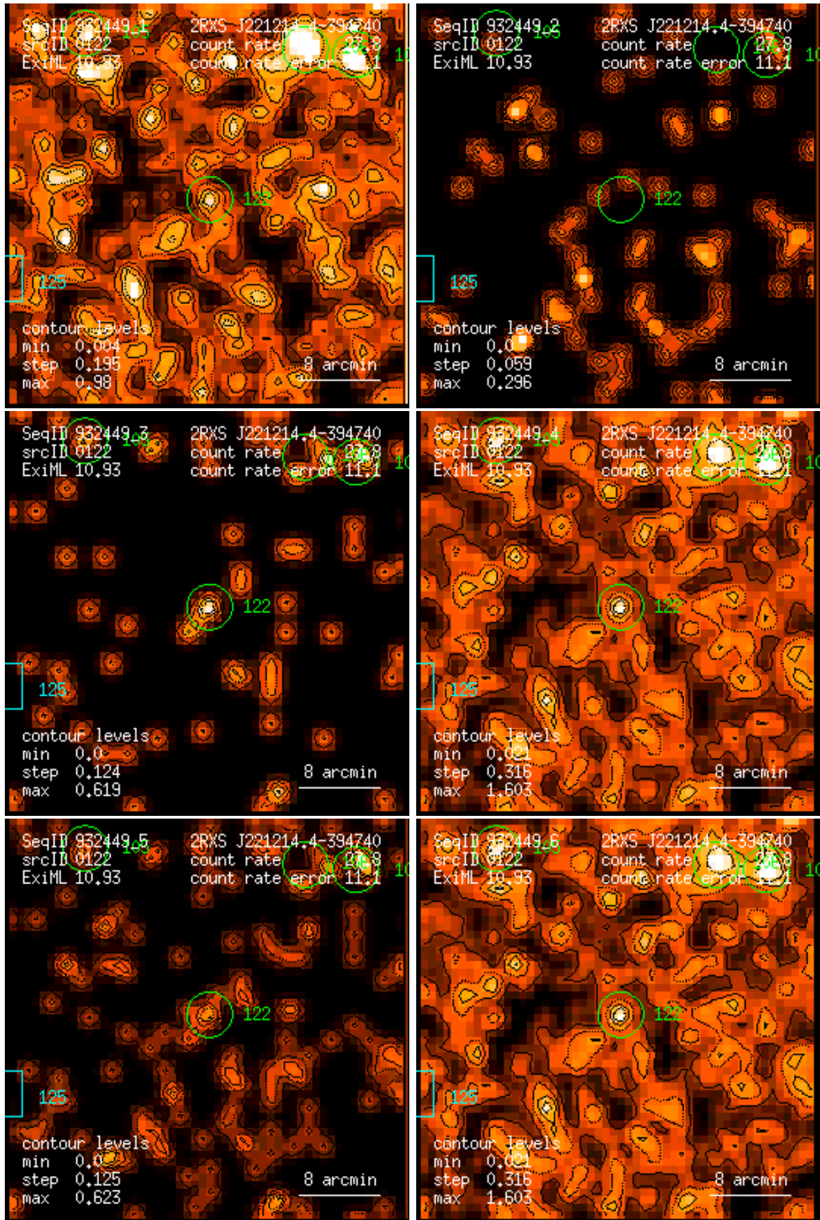
Figure 122: RASS 932449: detection 0122: band rate images, Gaussian filter: (1) PSPC channels 11 – 41, (2) 52 – 90, (3) 91 – 201, (4) 11 – 235, (5) 52 – 201, (6) 11 – 201. Broad band rates in counts/ks. Band rate contour levels in counts/ks/arcmin 2 .
