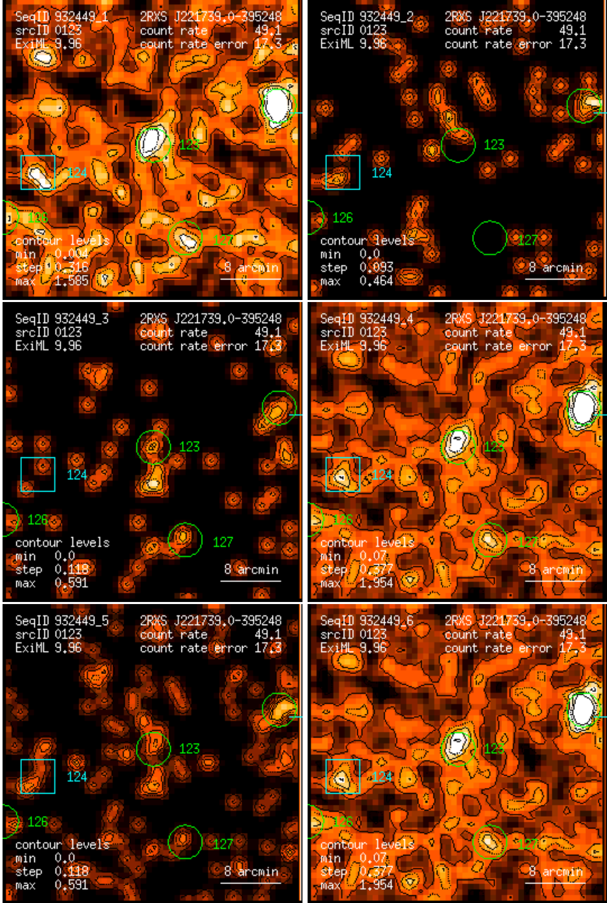
Figure 123: RASS 932449: detection 0123: band rate images, Gaussian filter: (1) PSPC channels 11 – 41, (2) 52 – 90, (3) 91 – 201, (4) 11 – 235, (5) 52 – 201, (6) 11 – 201. Broad band rates in counts/ks. Band rate contour levels in counts/ks/arcmin 2 .
