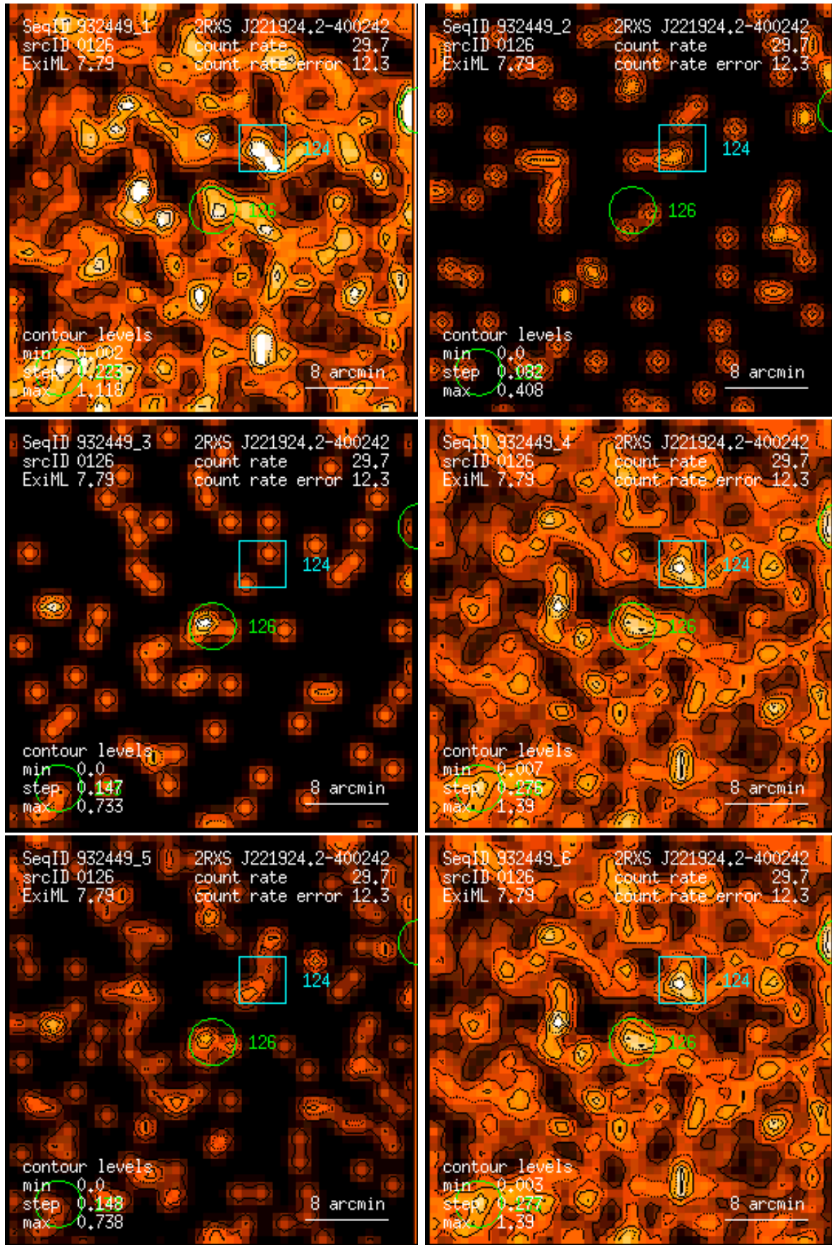
Figure 126: RASS 932449: detection 0126: band rate images, Gaussian filter: (1) PSPC channels 11 – 41, (2) 52 – 90, (3) 91 – 201, (4) 11 – 235, (5) 52 – 201, (6) 11 – 201. Broad band rates in counts/ks. Band rate contour levels in counts/ks/arcmin 2 .
