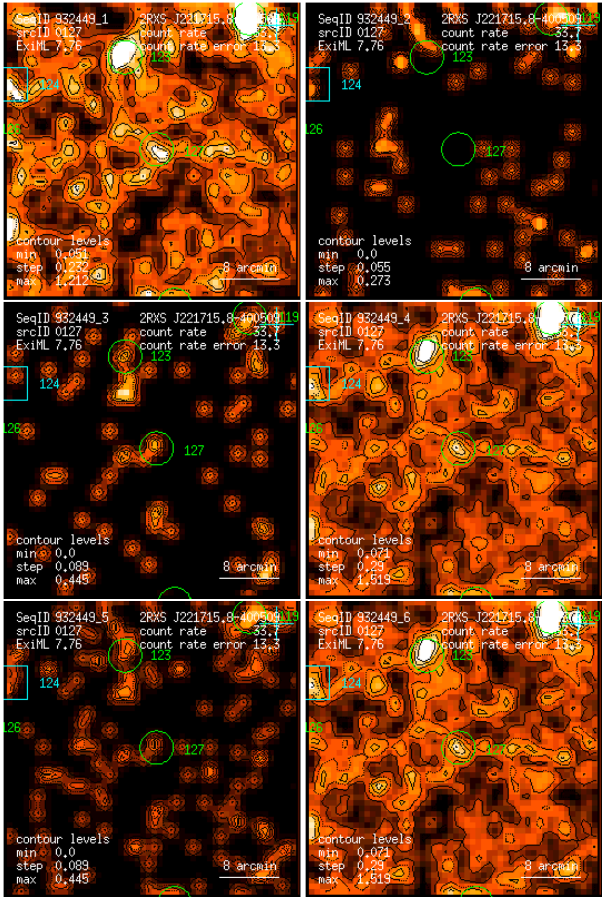
Figure 127: RASS 932449: detection 0127: band rate images, Gaussian filter: (1) PSPC channels 11 – 41, (2) 52 – 90, (3) 91 – 201, (4) 11 – 235, (5) 52 – 201, (6) 11 – 201. Broad band rates in counts/ks. Band rate contour levels in counts/ks/arcmin 2 .
