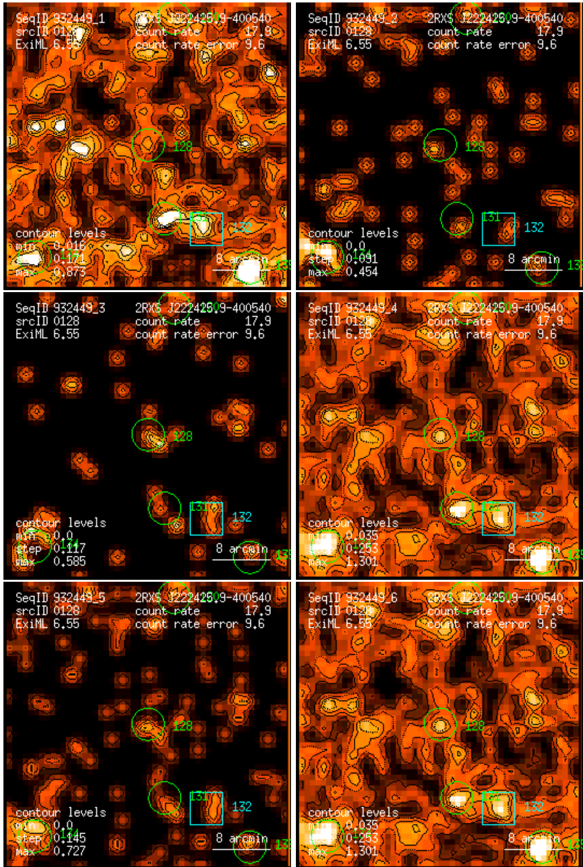
Figure 128: RASS 932449: detection 0128: band rate images, Gaussian filter: (1) PSPC channels 11 – 41, (2) 52 – 90, (3) 91 – 201, (4) 11 – 235, (5) 52 – 201, (6) 11 – 201. Broad band rates in counts/ks. Band rate contour levels in counts/ks/arcmin 2 .
