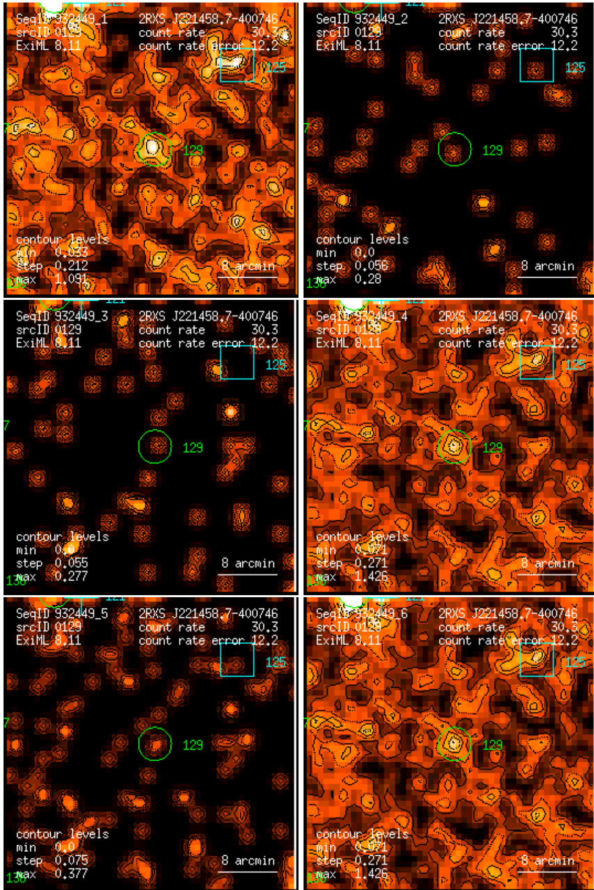
Figure 129: RASS 932449: detection 0129: band rate images, Gaussian filter: (1) PSPC channels 11 – 41, (2) 52 – 90, (3) 91 – 201, (4) 11 – 235, (5) 52 – 201, (6) 11 – 201. Broad band rates in counts/ks. Band rate contour levels in counts/ks/arcmin 2 .
