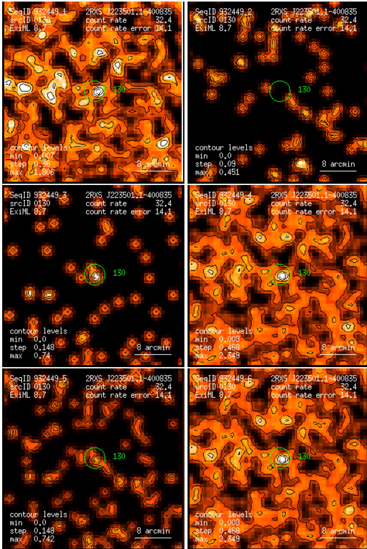
Figure 130: RASS 932449: detection 0130: band rate images, Gaussian filter: (1) PSPC channels 11 – 41, (2) 52 – 90, (3) 91 – 201, (4) 11 – 235, (5) 52 – 201, (6) 11 – 201. Broad band rates in counts/ks. Band rate contour levels in counts/ks/arcmin 2 .
