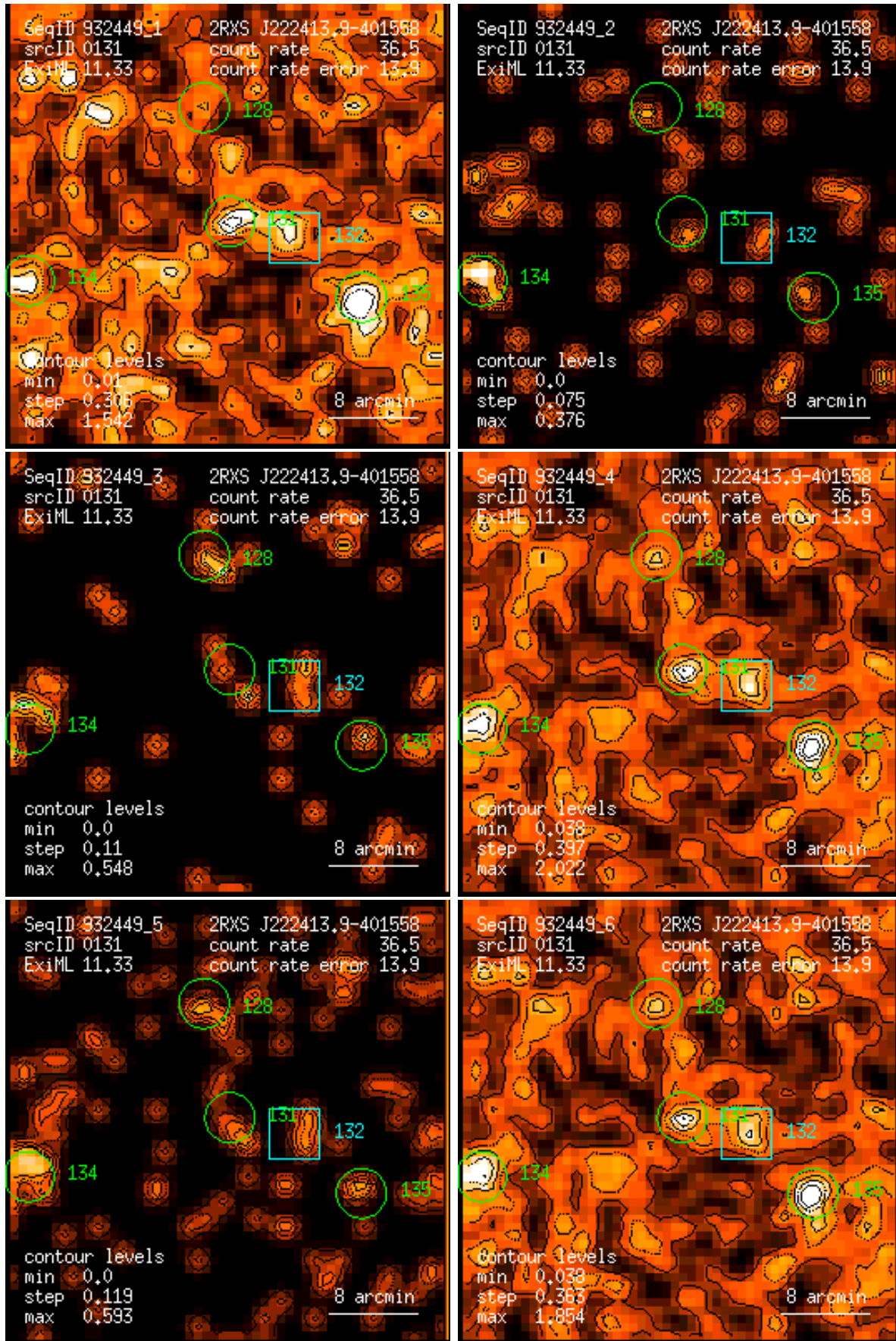
Figure 131: RASS 932449: detection 0131: band rate images, Gaussian filter: (1) PSPC channels 11 – 41, (2) 52 – 90, (3) 91 – 201, (4) 11 – 235, (5) 52 – 201, (6) 11 – 201. Broad band rates in counts/ks. Band rate contour levels in counts/ks/arcmin 2 .
