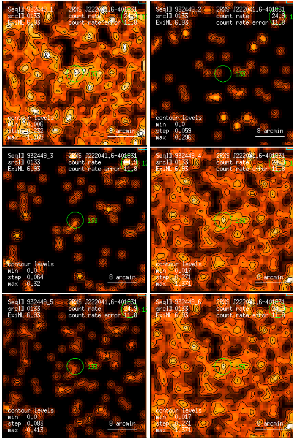
Figure 133: RASS 932449: detection 0133: band rate images, Gaussian filter: (1) PSPC channels 11 – 41, (2) 52 – 90, (3) 91 – 201, (4) 11 – 235, (5) 52 – 201, (6) 11 – 201. Broad band rates in counts/ks. Band rate contour levels in counts/ks/arcmin 2 .
