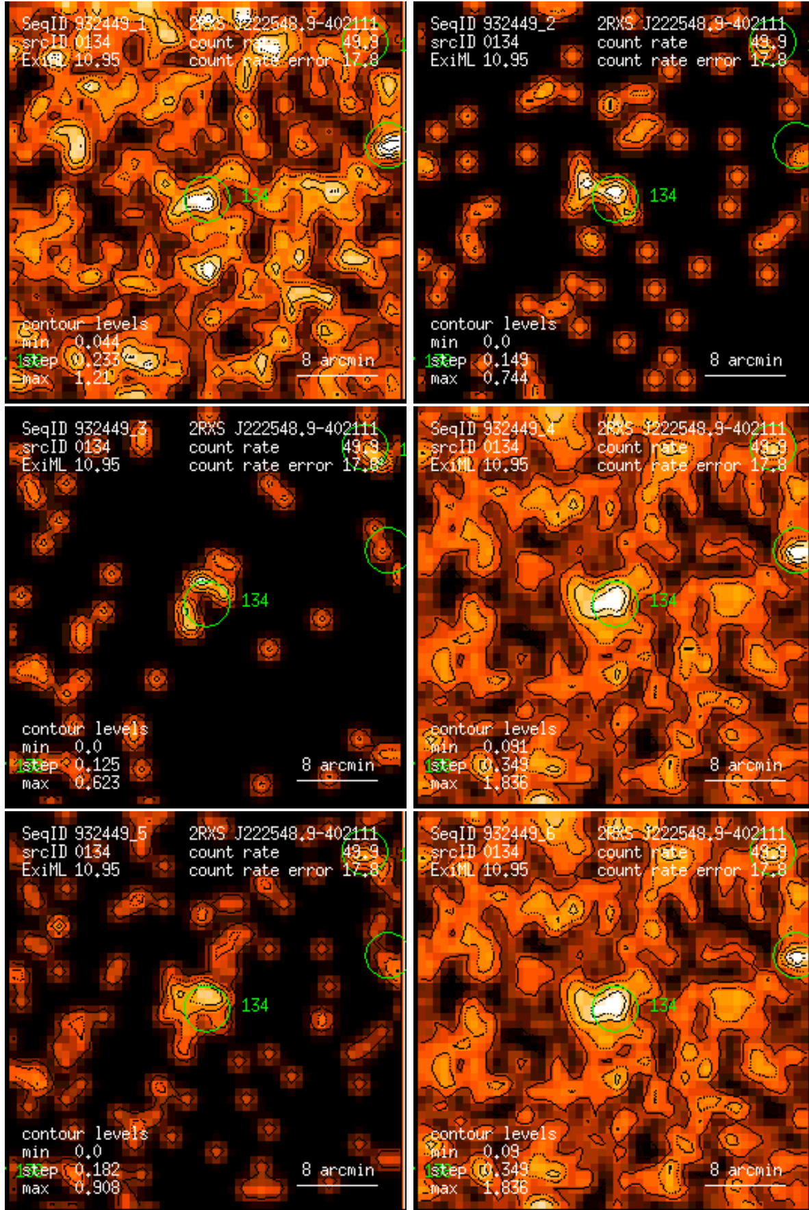
Figure 134: RASS 932449: detection 0134: band rate images, Gaussian filter: (1) PSPC channels 11 – 41, (2) 52 – 90, (3) 91 – 201, (4) 11 – 235, (5) 52 – 201, (6) 11 – 201. Broad band rates in counts/ks. Band rate contour levels in counts/ks/arcmin 2 .
