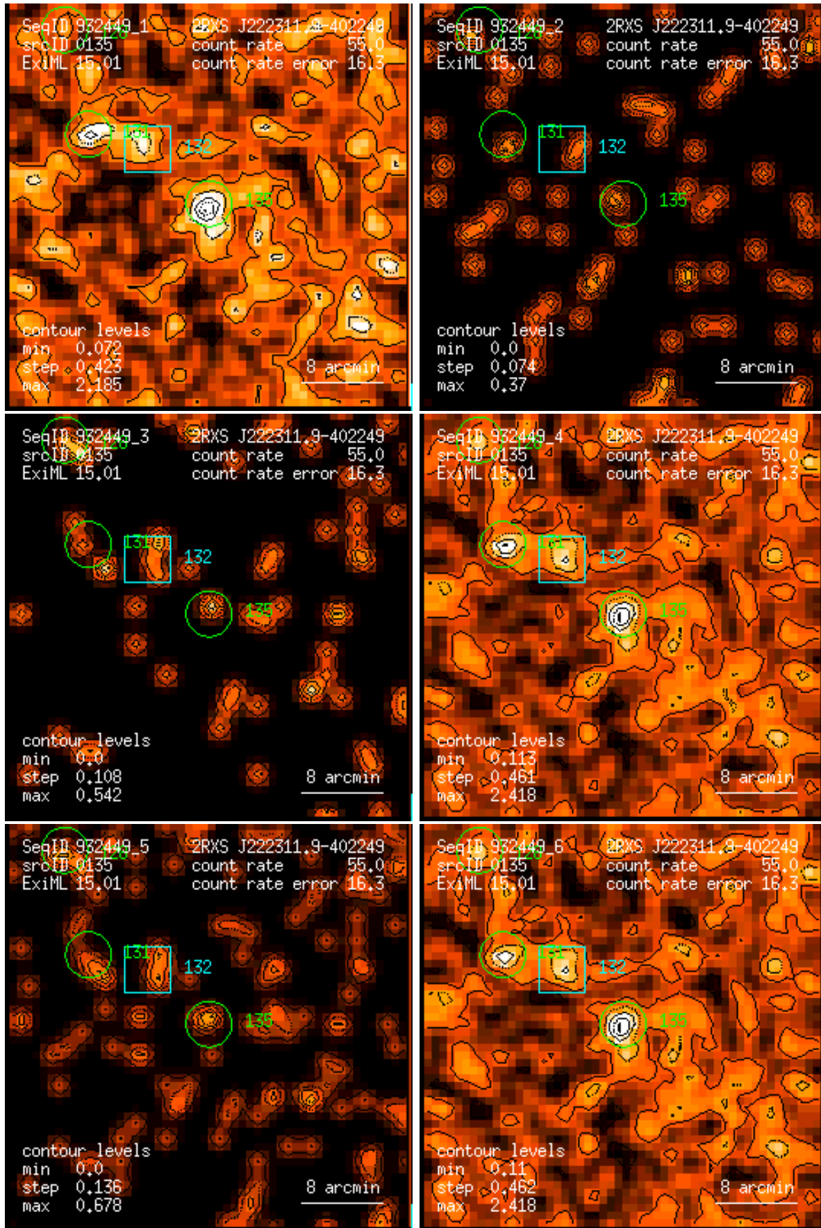
Figure 135: RASS 932449: detection 0135: band rate images, Gaussian filter: (1) PSPC channels 11 – 41, (2) 52 – 90, (3) 91 – 201, (4) 11 – 235, (5) 52 – 201, (6) 11 – 201. Broad band rates in counts/ks. Band rate contour levels in counts/ks/arcmin 2 .
