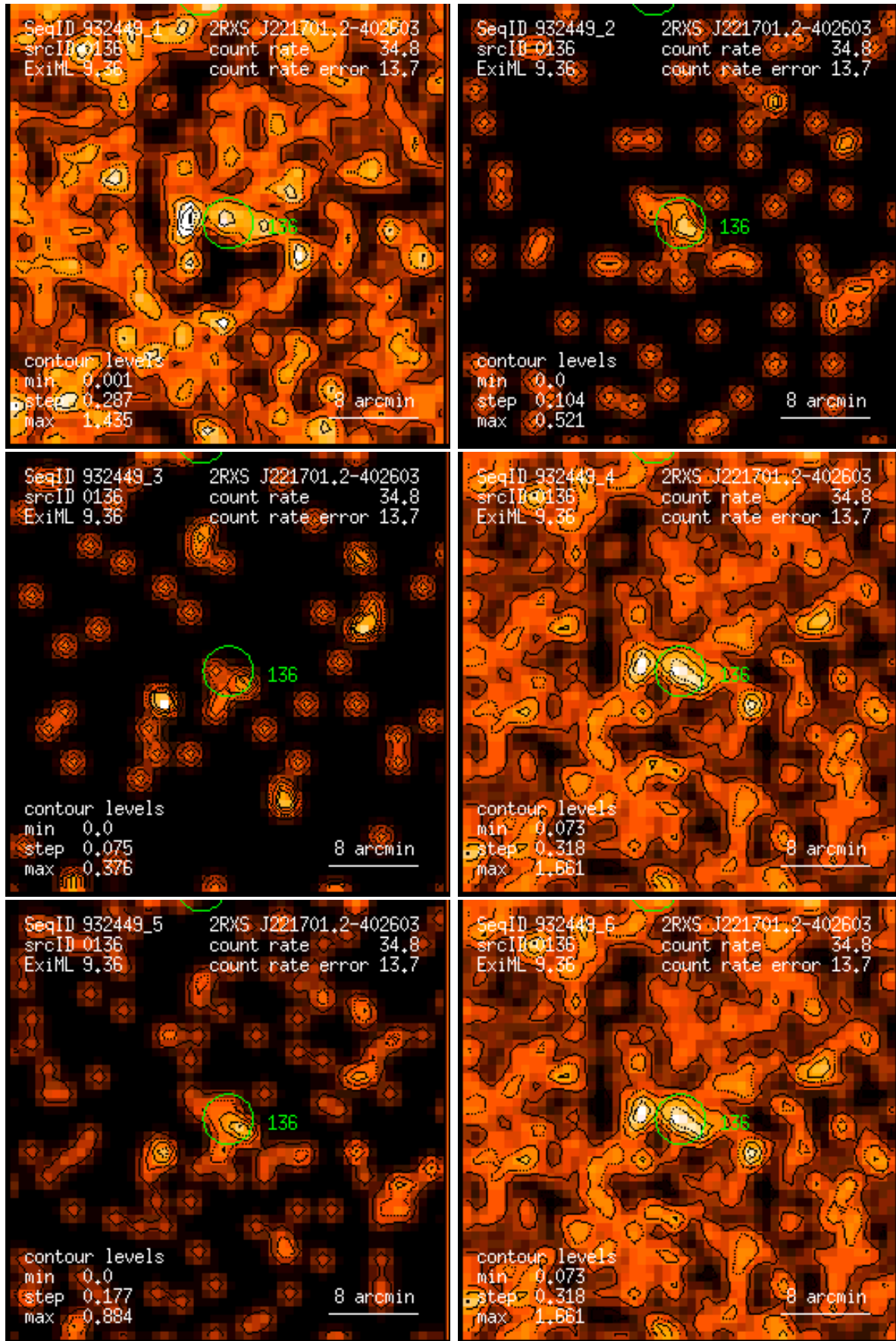
Figure 136: RASS 932449: detection 0136: band rate images, Gaussian filter: (1) PSPC channels 11 – 41, (2) 52 – 90, (3) 91 – 201, (4) 11 – 235, (5) 52 – 201, (6) 11 – 201. Broad band rates in counts/ks. Band rate contour levels in counts/ks/arcmin 2 .
