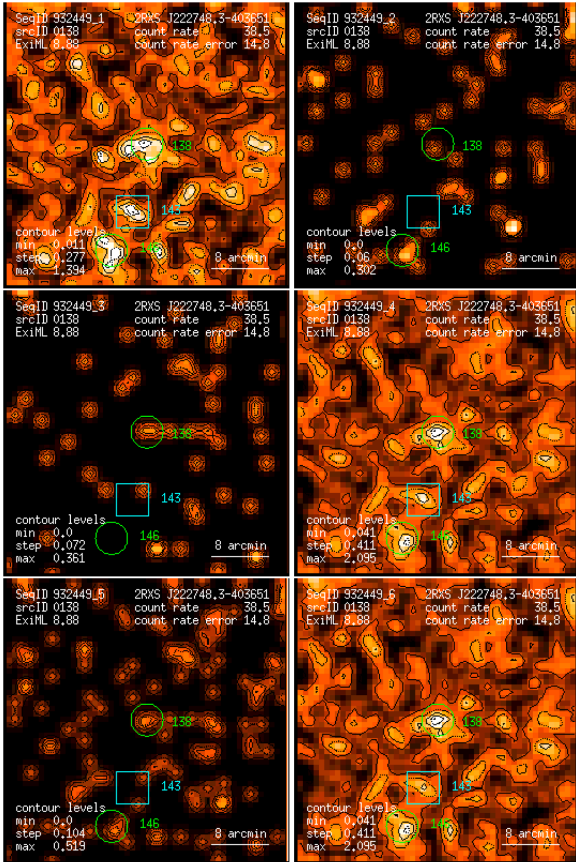
Figure 138: RASS 932449: detection 0138: band rate images, Gaussian filter: (1) PSPC channels 11 – 41, (2) 52 – 90, (3) 91 – 201, (4) 11 – 235, (5) 52 – 201, (6) 11 – 201. Broad band rates in counts/ks. Band rate contour levels in counts/ks/arcmin 2 .
