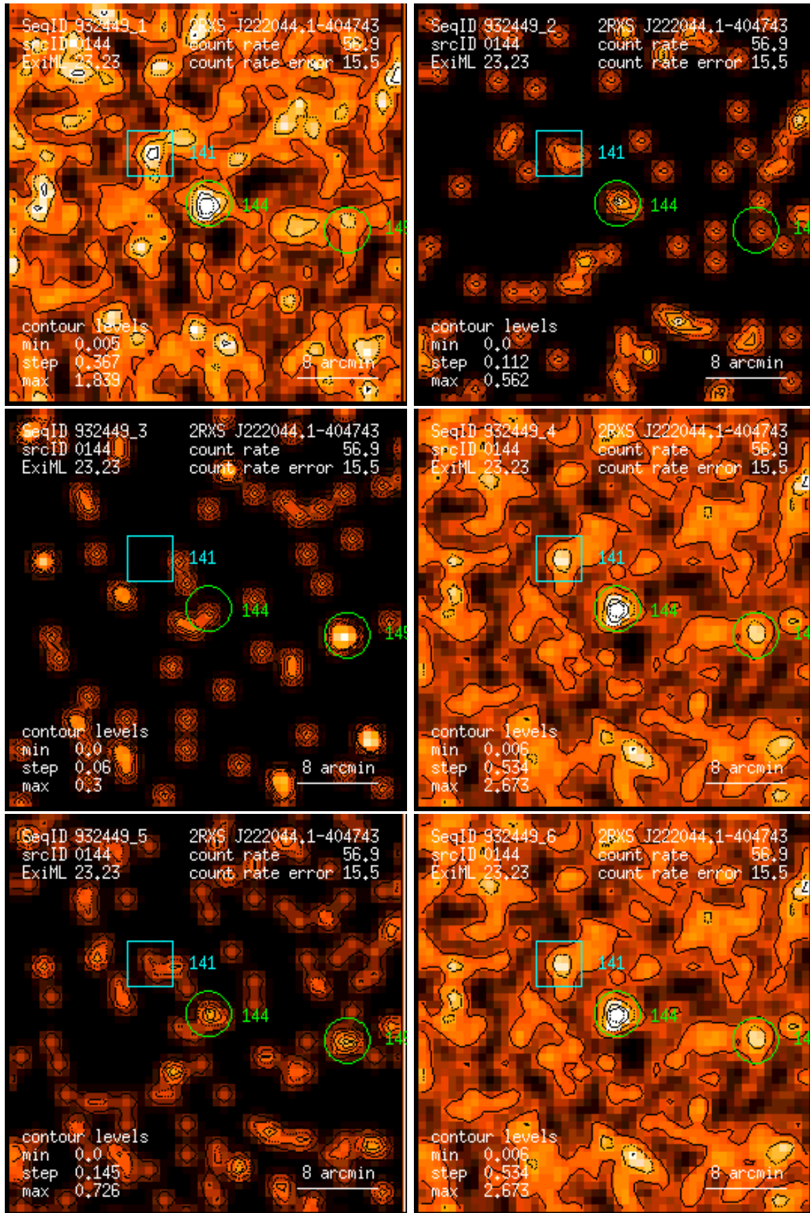
Figure 144: RASS 932449: detection 0144: band rate images, Gaussian filter: (1) PSPC channels 11 – 41, (2) 52 – 90, (3) 91 – 201, (4) 11 – 235, (5) 52 – 201, (6) 11 – 201. Broad band rates in counts/ks. Band rate contour levels in counts/ks/arcmin 2 .
