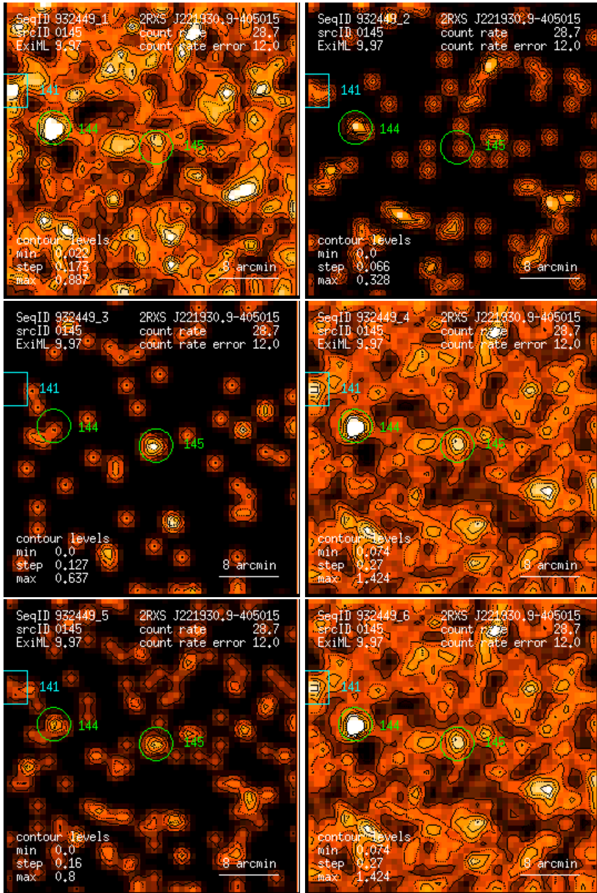
Figure 145: RASS 932449: detection 0145: band rate images, Gaussian filter: (1) PSPC channels 11 – 41, (2) 52 – 90, (3) 91 – 201, (4) 11 – 235, (5) 52 – 201, (6) 11 – 201. Broad band rates in counts/ks. Band rate contour levels in counts/ks/arcmin 2 .
