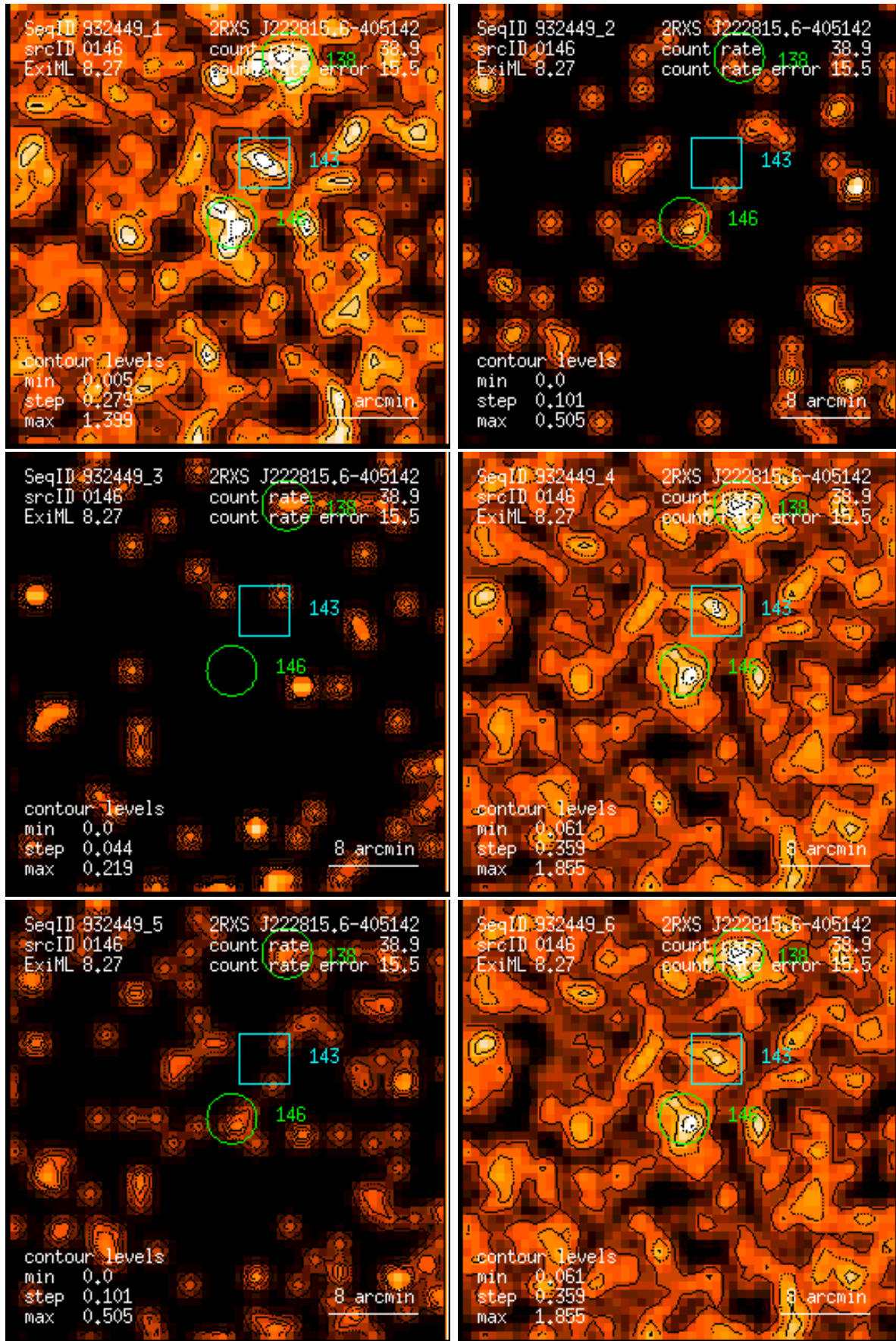
Figure 146: RASS 932449: detection 0146: band rate images, Gaussian filter: (1) PSPC channels 11 – 41, (2) 52 – 90, (3) 91 – 201, (4) 11 – 235, (5) 52 – 201, (6) 11 – 201. Broad band rates in counts/ks. Band rate contour levels in counts/ks/arcmin 2 .
