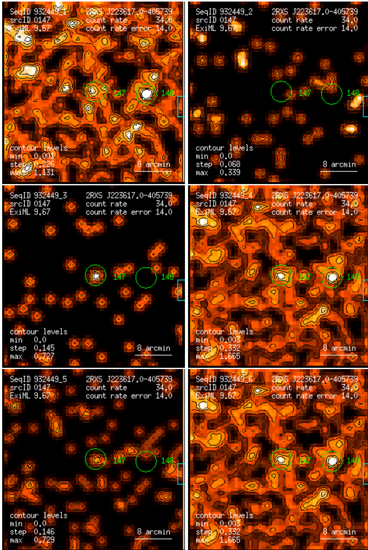
Figure 147: RASS 932449: detection 0147: band rate images, Gaussian filter: (1) PSPC channels 11 – 41, (2) 52 – 90, (3) 91 – 201, (4) 11 – 235, (5) 52 – 201, (6) 11 – 201. Broad band rates in counts/ks. Band rate contour levels in counts/ks/arcmin 2 .
