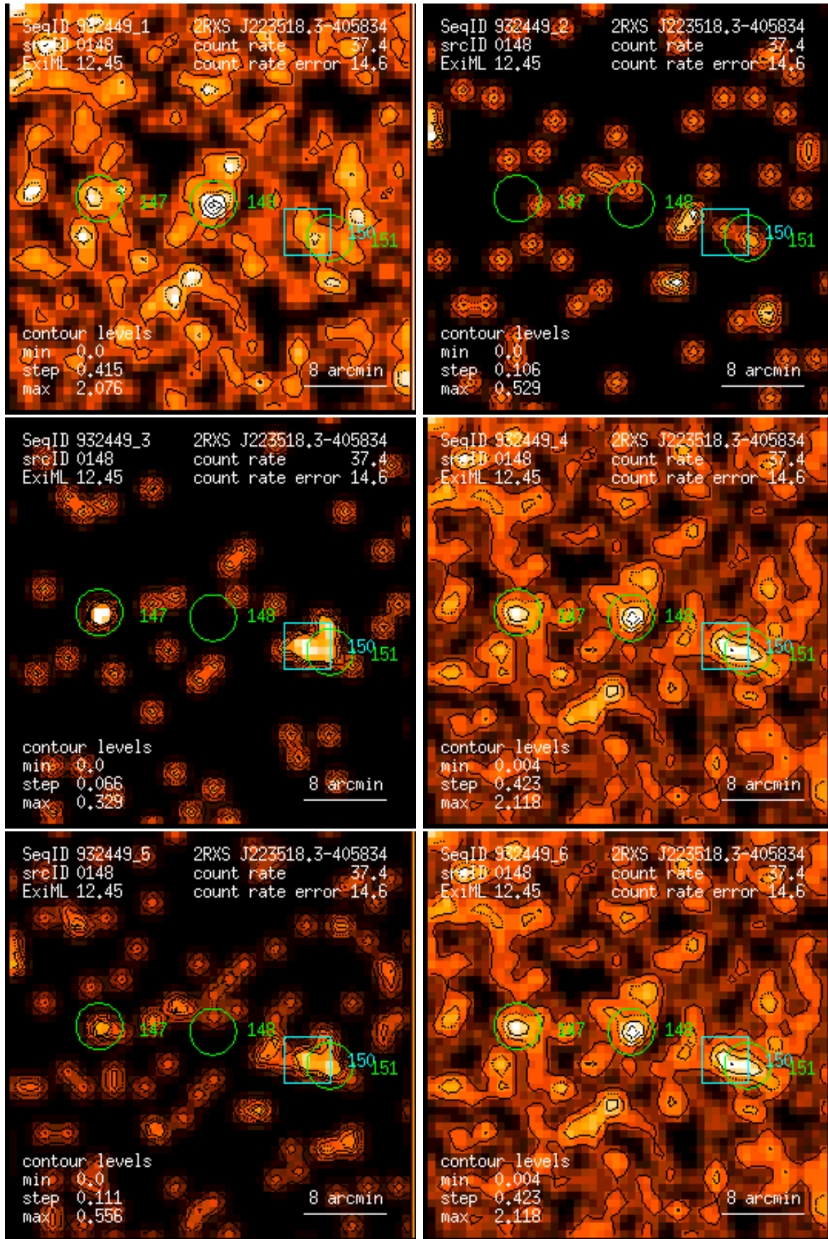
Figure 148: RASS 932449: detection 0148: band rate images, Gaussian filter: (1) PSPC channels 11 – 41, (2) 52 – 90, (3) 91 – 201, (4) 11 – 235, (5) 52 – 201, (6) 11 – 201. Broad band rates in counts/ks. Band rate contour levels in counts/ks/arcmin 2 .
