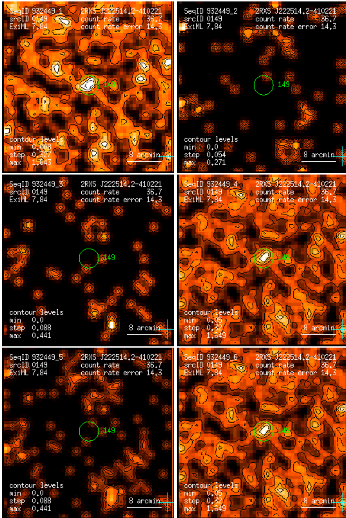
Figure 149: RASS 932449: detection 0149: band rate images, Gaussian filter: (1) PSPC channels 11 – 41, (2) 52 – 90, (3) 91 – 201, (4) 11 – 235, (5) 52 – 201, (6) 11 – 201. Broad band rates in counts/ks. Band rate contour levels in counts/ks/arcmin 2 .
