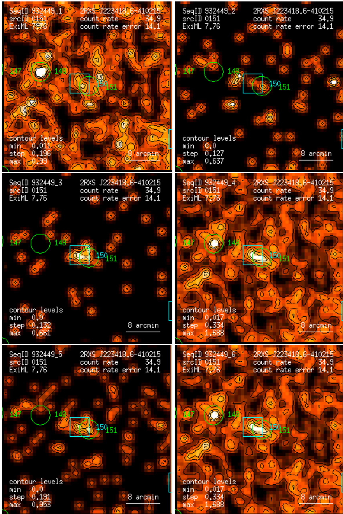
Figure 151: RASS 932449: detection 0151: band rate images, Gaussian filter: (1) PSPC channels 11 – 41, (2) 52 – 90, (3) 91 – 201, (4) 11 – 235, (5) 52 – 201, (6) 11 – 201. Broad band rates in counts/ks. Band rate contour levels in counts/ks/arcmin 2 .
