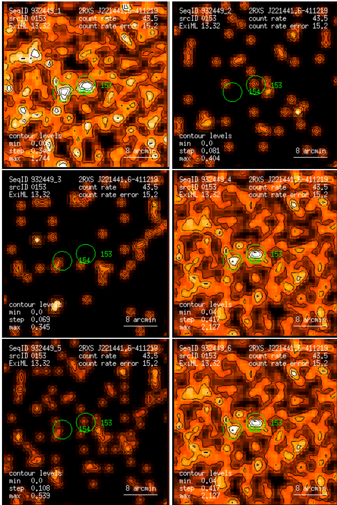
Figure 153: RASS 932449: detection 0153: band rate images, Gaussian filter: (1) PSPC channels 11 – 41, (2) 52 – 90, (3) 91 – 201, (4) 11 – 235, (5) 52 – 201, (6) 11 – 201. Broad band rates in counts/ks. Band rate contour levels in counts/ks/arcmin 2 .
