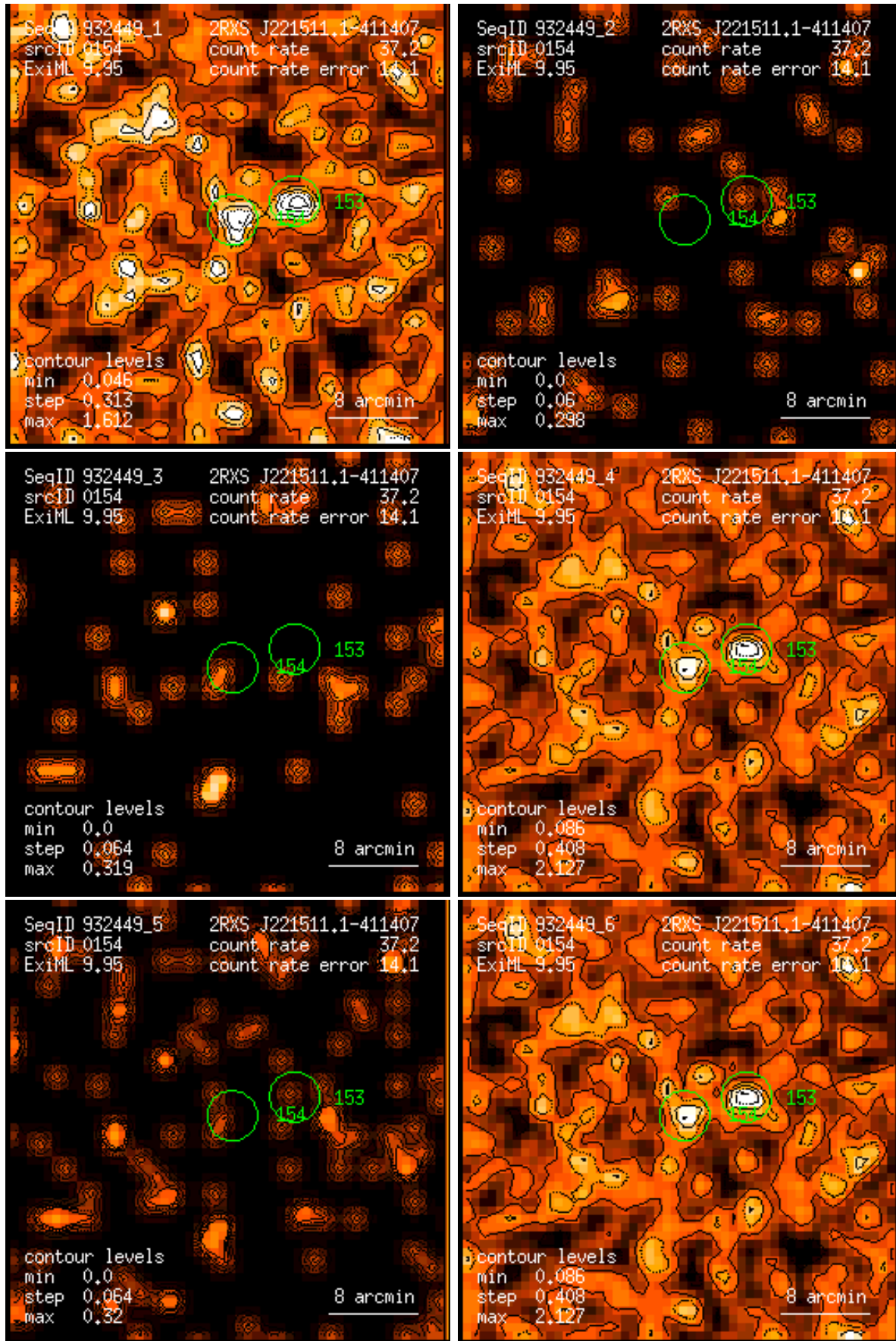
Figure 154: RASS 932449: detection 0154: band rate images, Gaussian filter: (1) PSPC channels 11 – 41, (2) 52 – 90, (3) 91 – 201, (4) 11 – 235, (5) 52 – 201, (6) 11 – 201. Broad band rates in counts/ks. Band rate contour levels in counts/ks/arcmin 2 .
