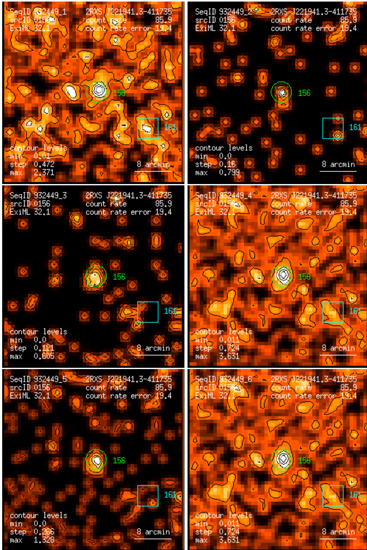
Figure 156: RASS 932449: detection 0156: band rate images, Gaussian filter: (1) PSPC channels 11 – 41, (2) 52 – 90, (3) 91 – 201, (4) 11 – 235, (5) 52 – 201, (6) 11 – 201. Broad band rates in counts/ks. Band rate contour levels in counts/ks/arcmin 2 .
