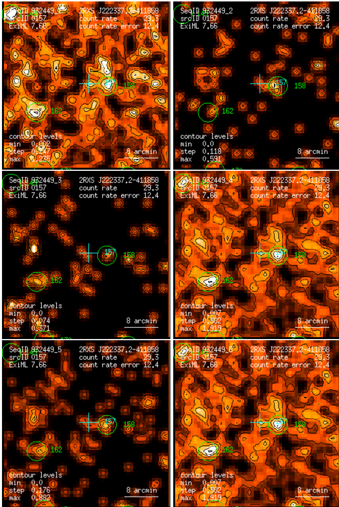
Figure 157: RASS 932449: detection 0157: band rate images, Gaussian filter: (1) PSPC channels 11 – 41, (2) 52 – 90, (3) 91 – 201, (4) 11 – 235, (5) 52 – 201, (6) 11 – 201. Broad band rates in counts/ks. Band rate contour levels in counts/ks/arcmin 2 .
