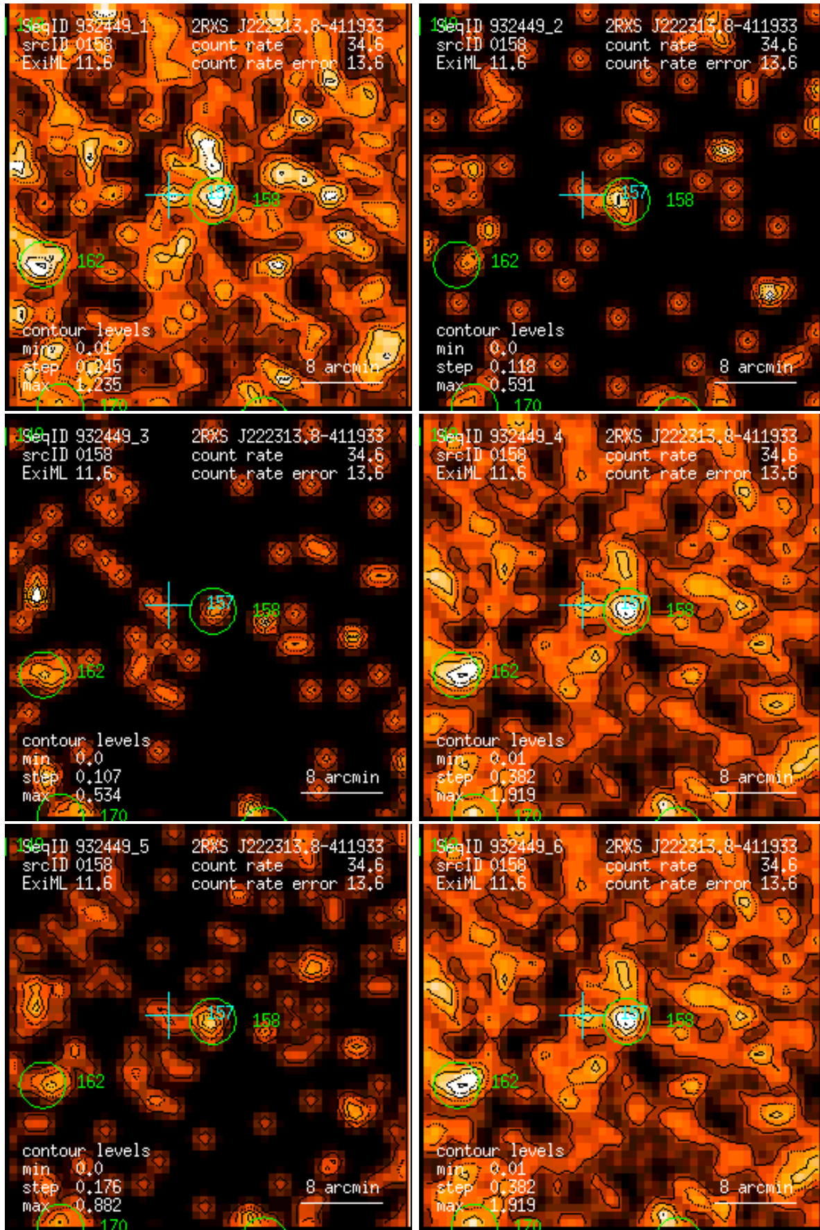
Figure 158: RASS 932449: detection 0158: band rate images, Gaussian filter: (1) PSPC channels 11 – 41, (2) 52 – 90, (3) 91 – 201, (4) 11 – 235, (5) 52 – 201, (6) 11 – 201. Broad band rates in counts/ks. Band rate contour levels in counts/ks/arcmin 2 .
