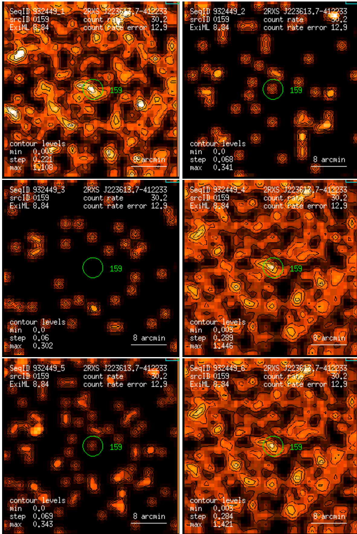
Figure 159: RASS 932449: detection 0159: band rate images, Gaussian filter: (1) PSPC channels 11 – 41, (2) 52 – 90, (3) 91 – 201, (4) 11 – 235, (5) 52 – 201, (6) 11 – 201. Broad band rates in counts/ks. Band rate contour levels in counts/ks/arcmin 2 .
