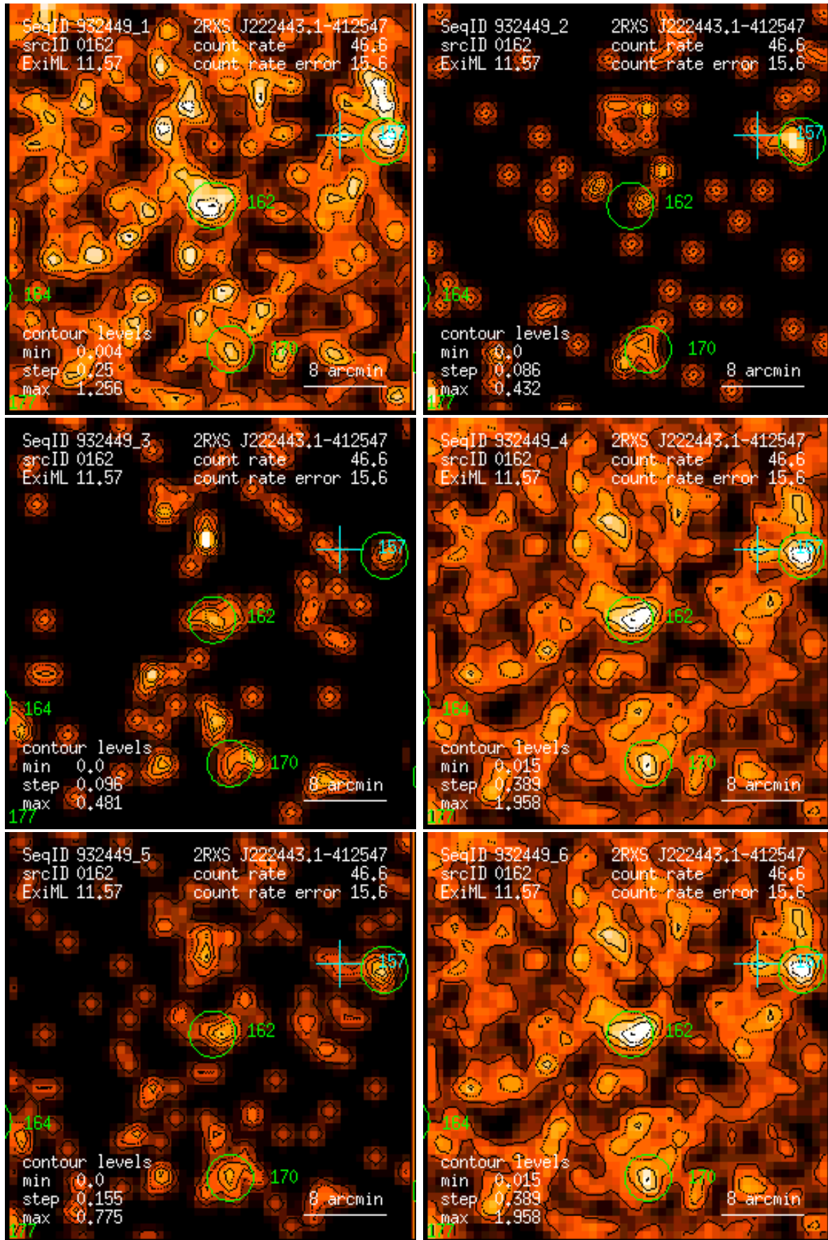
Figure 162: RASS 932449: detection 0162: band rate images, Gaussian filter: (1) PSPC channels 11 – 41, (2) 52 – 90, (3) 91 – 201, (4) 11 – 235, (5) 52 – 201, (6) 11 – 201. Broad band rates in counts/ks. Band rate contour levels in counts/ks/arcmin 2 .
