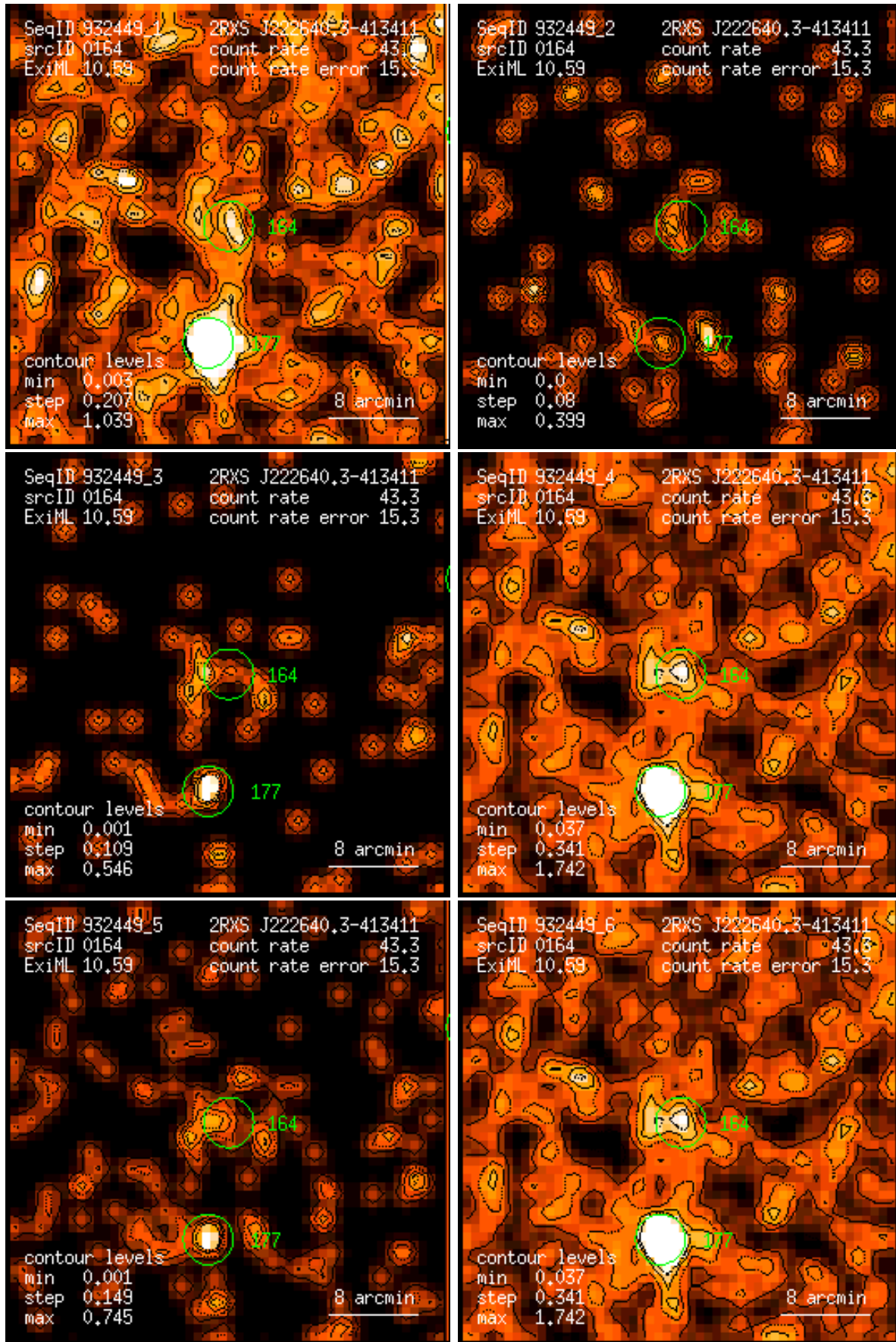
Figure 164: RASS 932449: detection 0164: band rate images, Gaussian filter: (1) PSPC channels 11 – 41, (2) 52 – 90, (3) 91 – 201, (4) 11 – 235, (5) 52 – 201, (6) 11 – 201. Broad band rates in counts/ks. Band rate contour levels in counts/ks/arcmin 2 .
