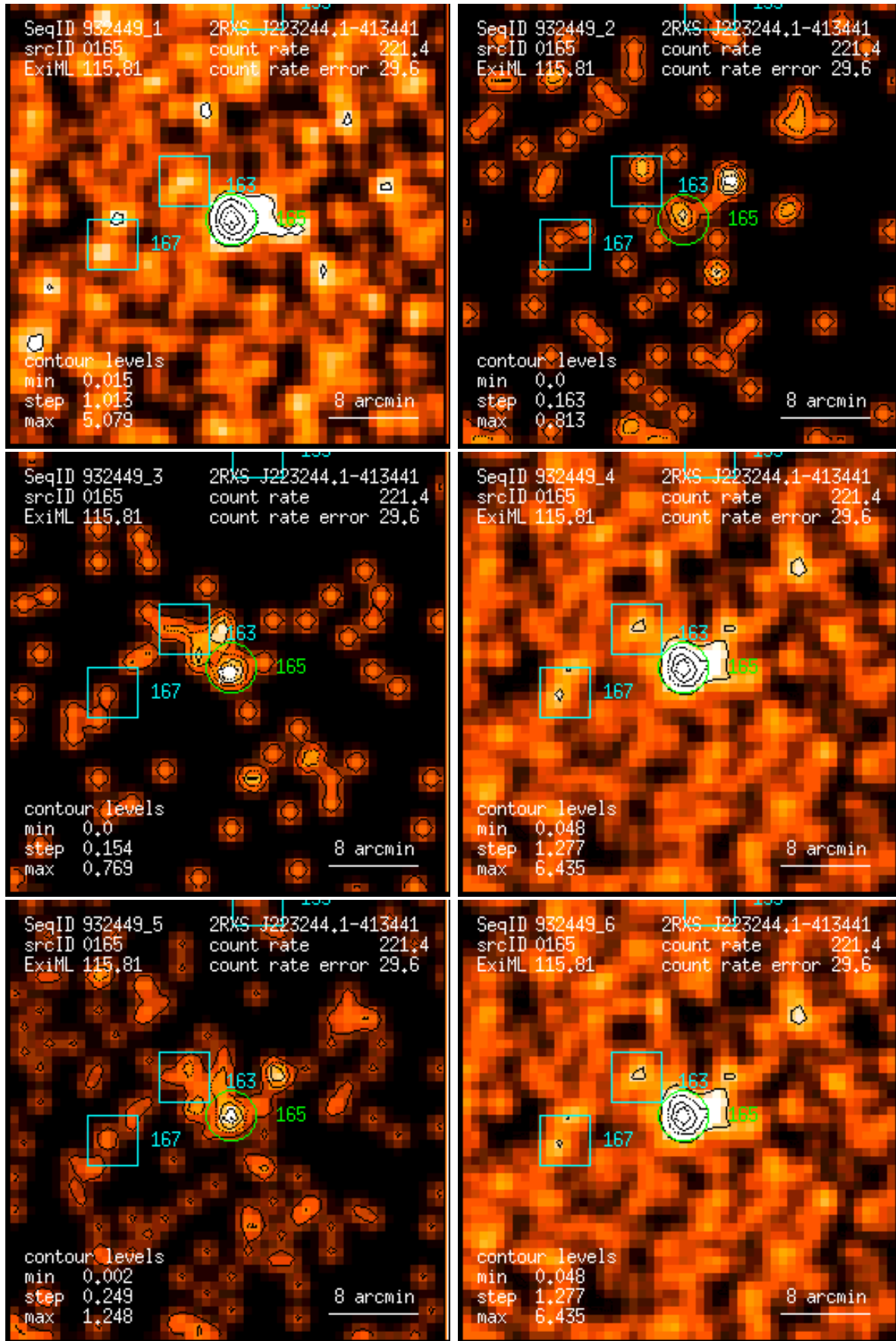
Figure 165: RASS 932449: detection 0165: band rate images, Gaussian filter: (1) PSPC channels 11 – 41, (2) 52 – 90, (3) 91 – 201, (4) 11 – 235, (5) 52 – 201, (6) 11 – 201. Broad band rates in counts/ks. Band rate contour levels in counts/ks/arcmin 2 .
