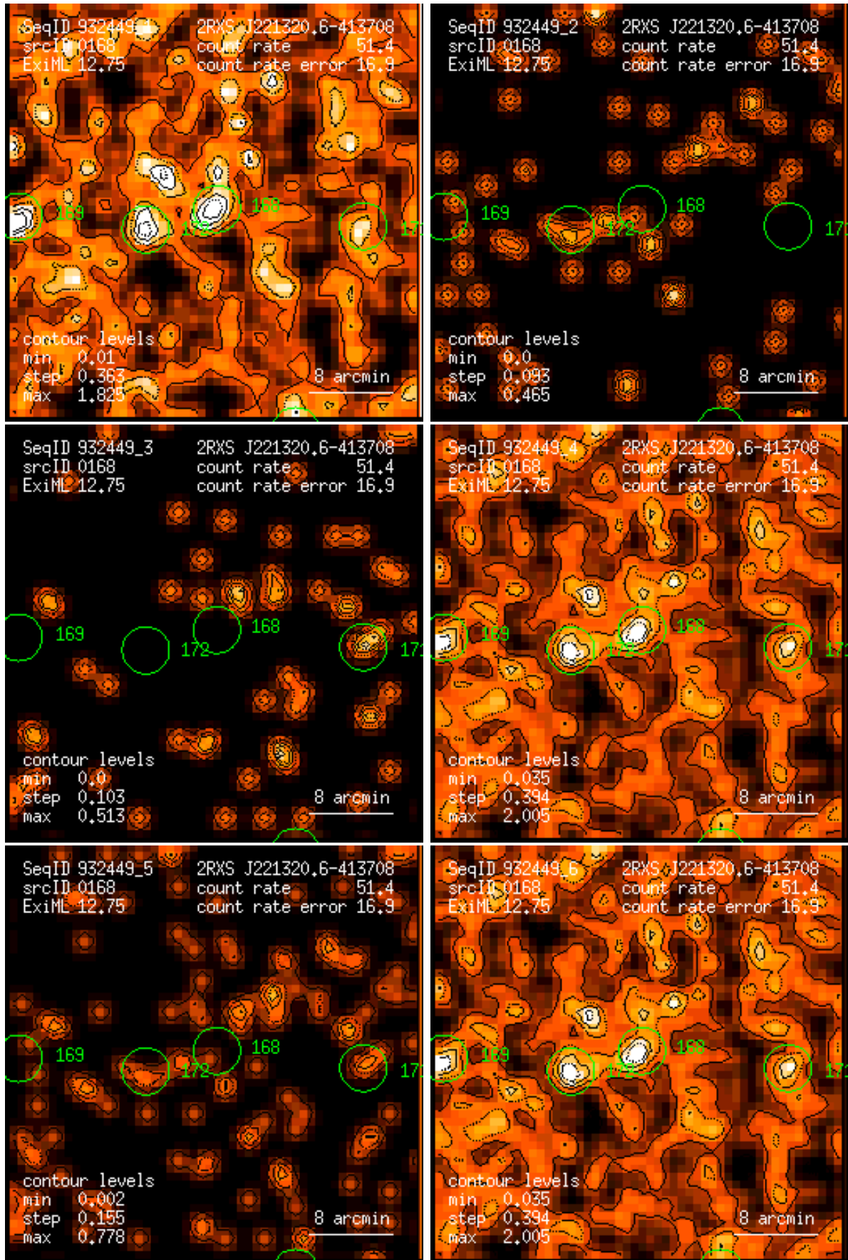
Figure 168: RASS 932449: detection 0168: band rate images, Gaussian filter: (1) PSPC channels 11 – 41, (2) 52 – 90, (3) 91 – 201, (4) 11 – 235, (5) 52 – 201, (6) 11 – 201. Broad band rates in counts/ks. Band rate contour levels in counts/ks/arcmin 2 .
