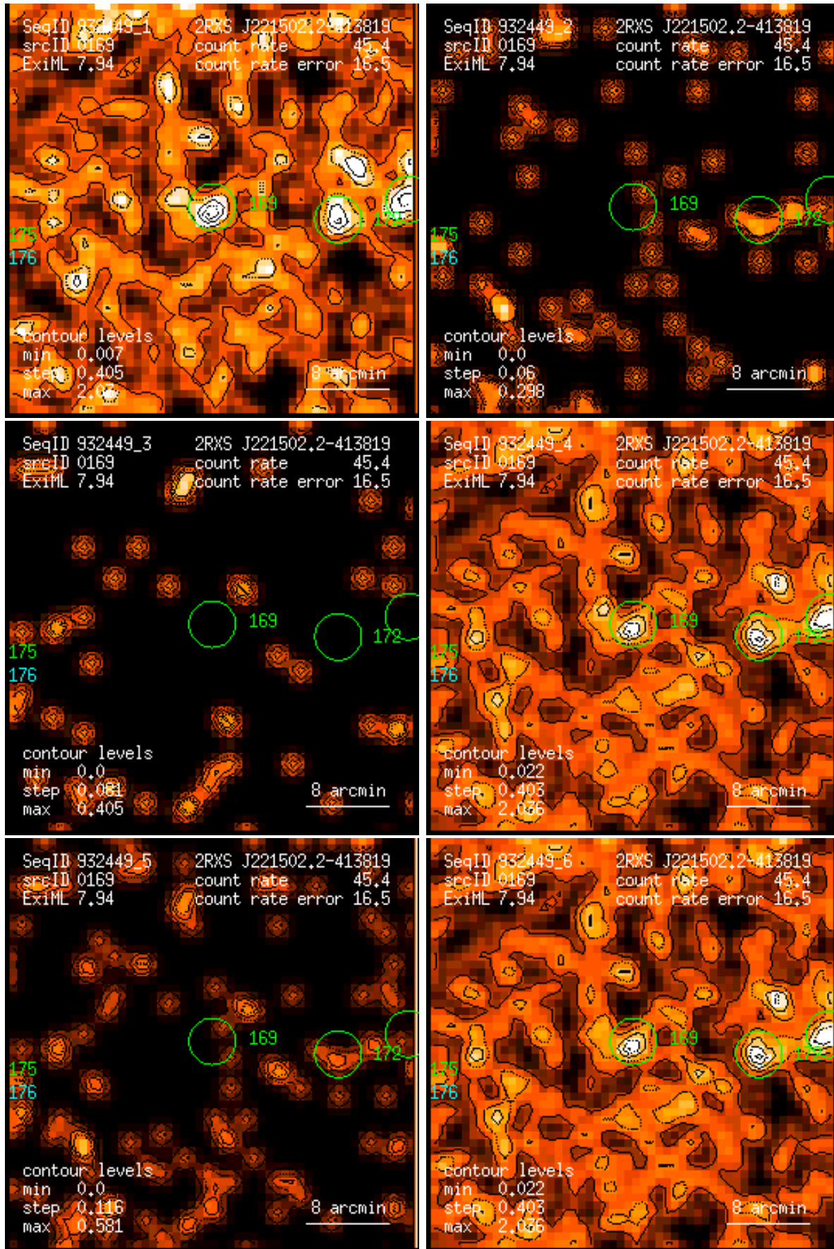
Figure 169: RASS 932449: detection 0169: band rate images, Gaussian filter: (1) PSPC channels 11 – 41, (2) 52 – 90, (3) 91 – 201, (4) 11 – 235, (5) 52 – 201, (6) 11 – 201. Broad band rates in counts/ks. Band rate contour levels in counts/ks/arcmin 2 .
