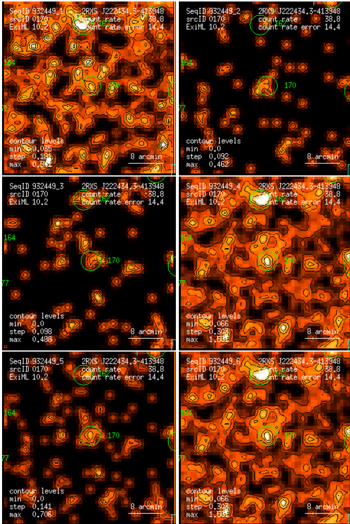
Figure 170: RASS 932449: detection 0170: band rate images, Gaussian filter: (1) PSPC channels 11 – 41, (2) 52 – 90, (3) 91 – 201, (4) 11 – 235, (5) 52 – 201, (6) 11 – 201. Broad band rates in counts/ks. Band rate contour levels in counts/ks/arcmin 2 .
