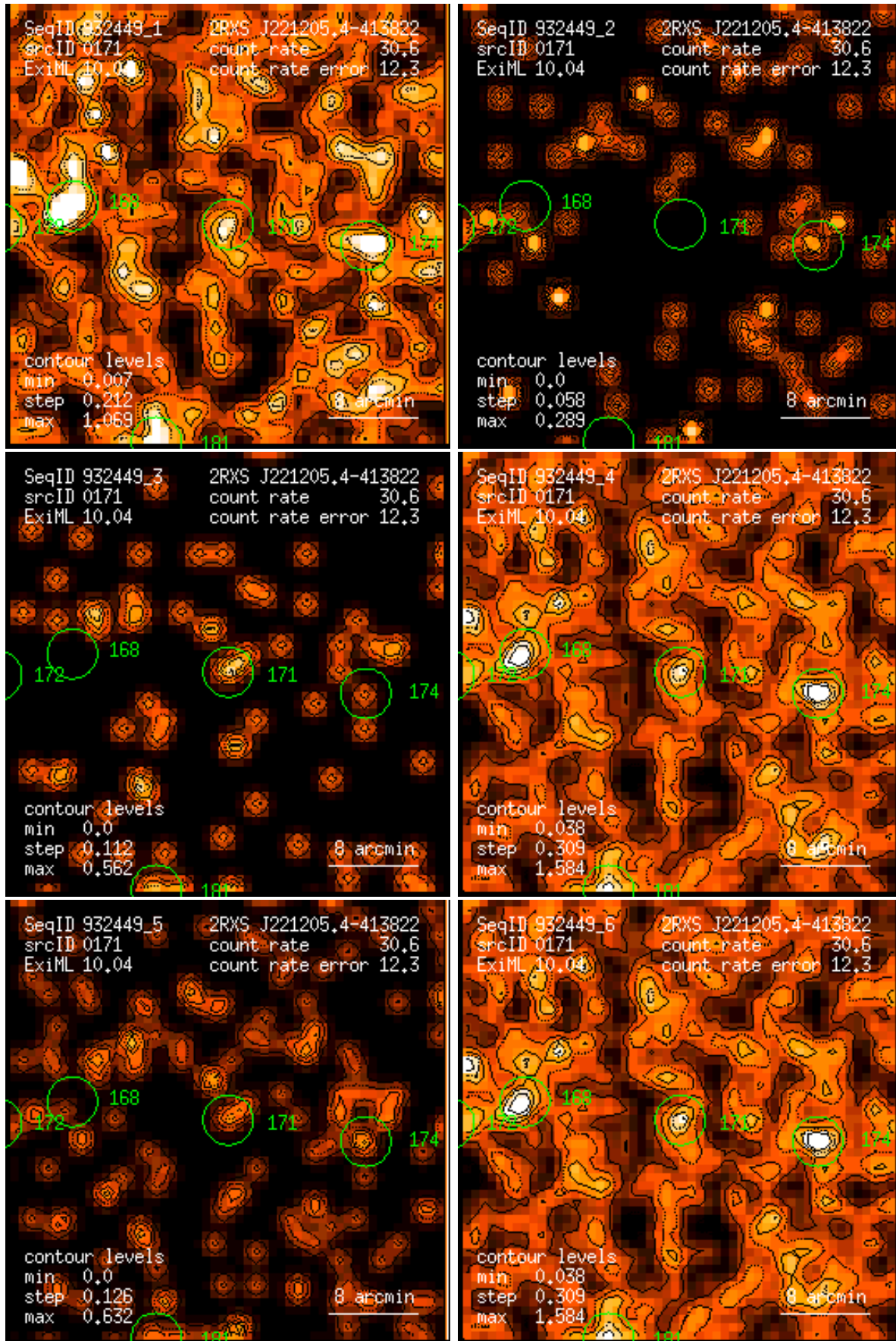
Figure 171: RASS 932449: detection 0171: band rate images, Gaussian filter: (1) PSPC channels 11 – 41, (2) 52 – 90, (3) 91 – 201, (4) 11 – 235, (5) 52 – 201, (6) 11 – 201. Broad band rates in counts/ks. Band rate contour levels in counts/ks/arcmin 2 .
